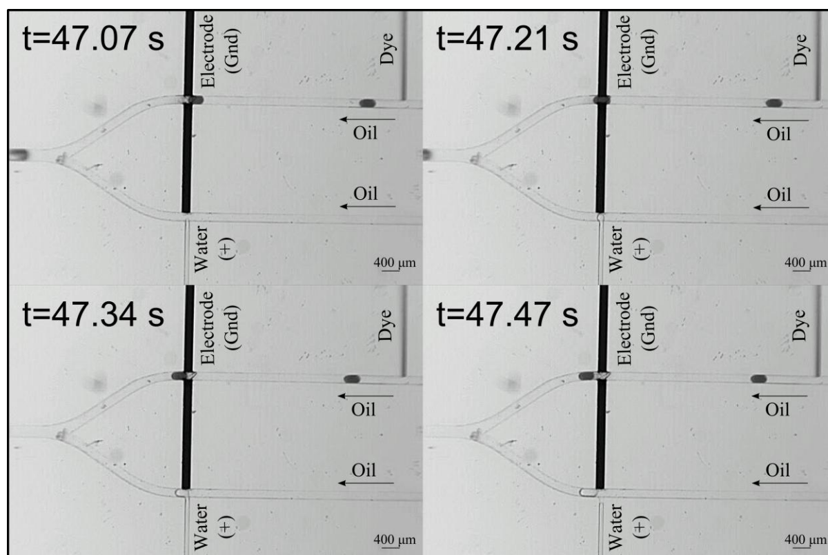
Figure S4: Generation of a water droplet as amaranth droplet passes a pair of electrodes ( V_{app} : 500 V)
