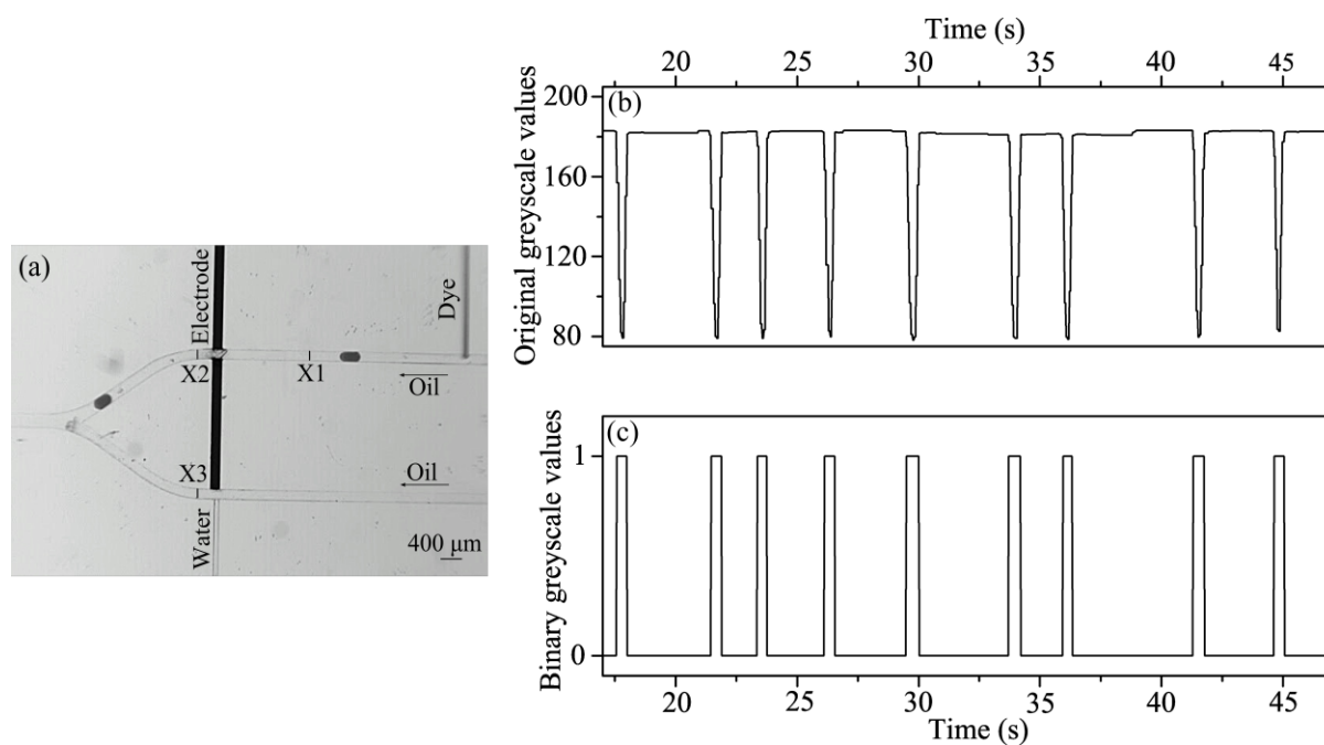
Figure S3: (a) Position of detection windows (i.e. X1, X2 and X3) and an example of light intensity values (b) before and (c) after image processing
