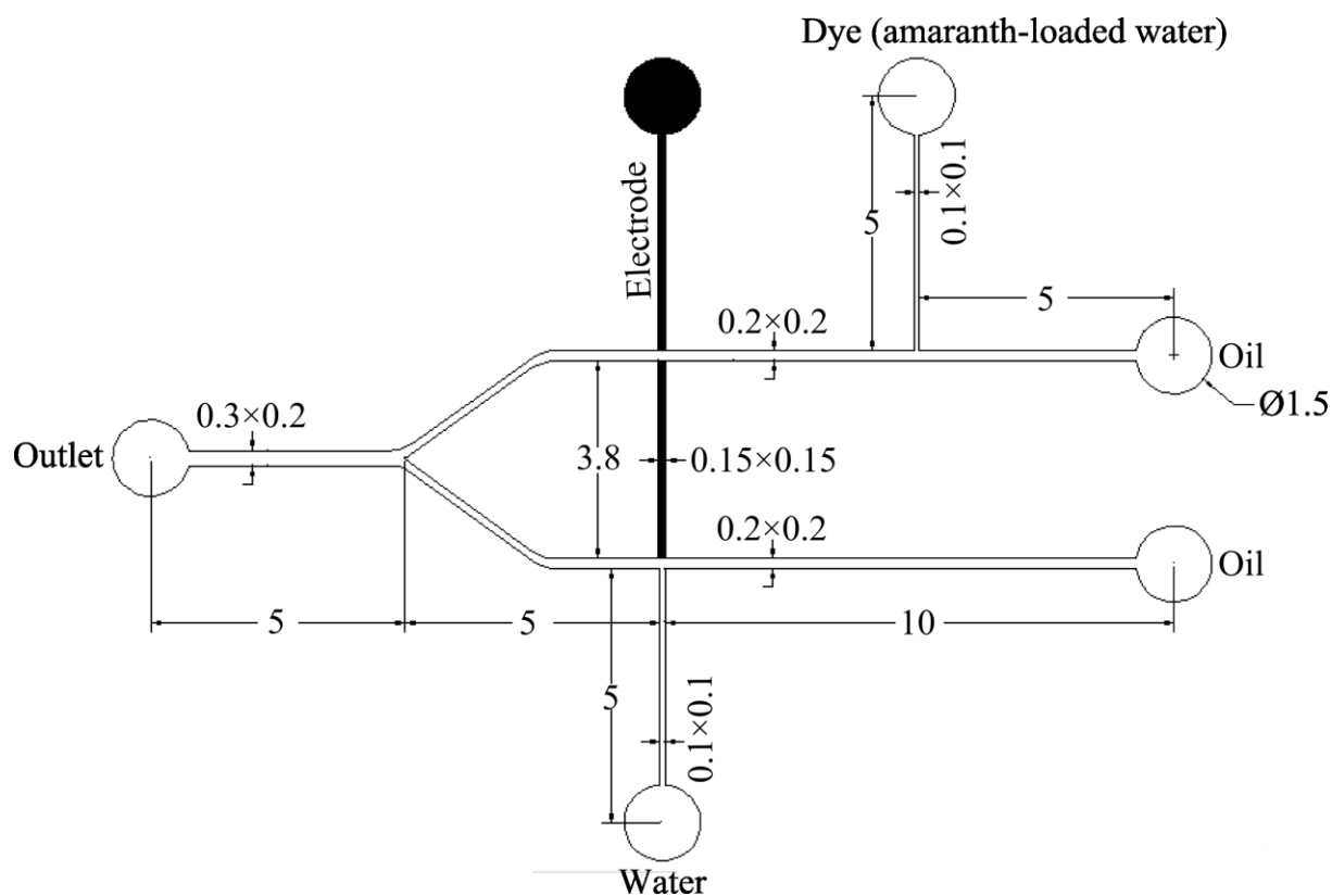
Figure S1: Layout along with dimensions of the miniaturised self-synchronised droplet production device (all dimensions are in mm)
