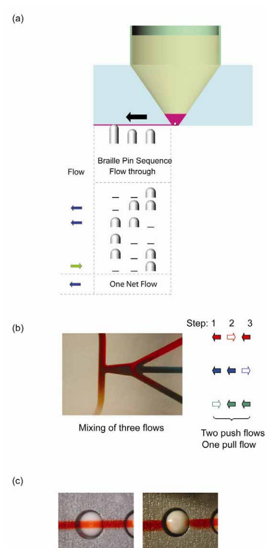
Figure 2. The actuation of the Braille for (a) pumping (flow through), (b) mixing, and (3) valve.
