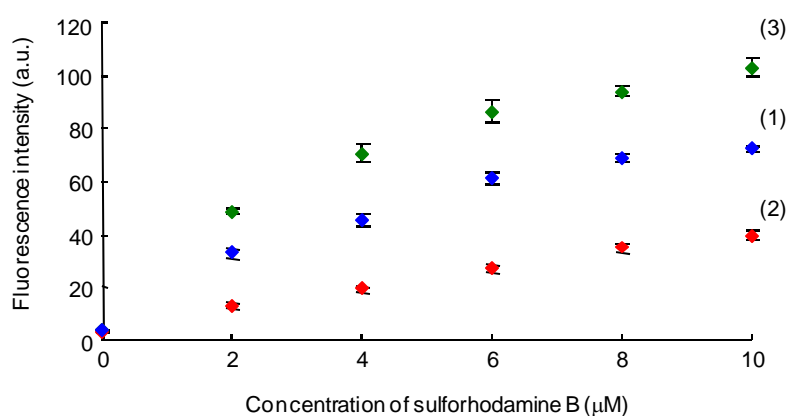
Figure S1 Calibration curves of sulforhodamine B solutions using different CPCs. (1)Conventional CPC, (2)Bulk modified CPC, (3)Surface modified CPC (Error bar represents relative standard deviation (n=3))
