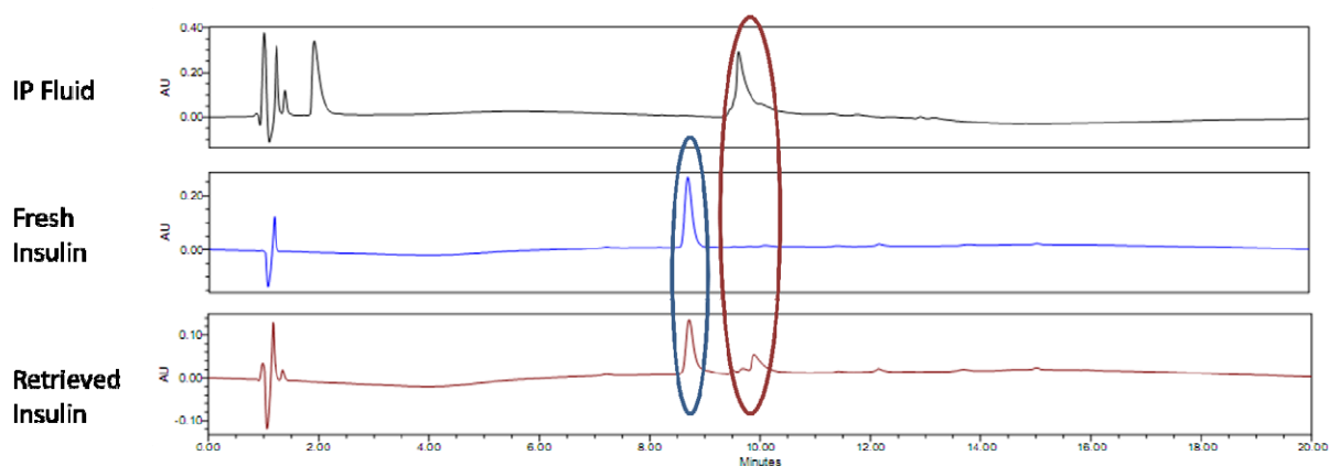
Fig. S2 – RP-HPLC chromatogram of soluble insulin from retrieved microdevices after 15 days of in vivo implantation compared with fresh human recombinant insulin and intraperitoneal (IP) fluid with endogenous proteins.
