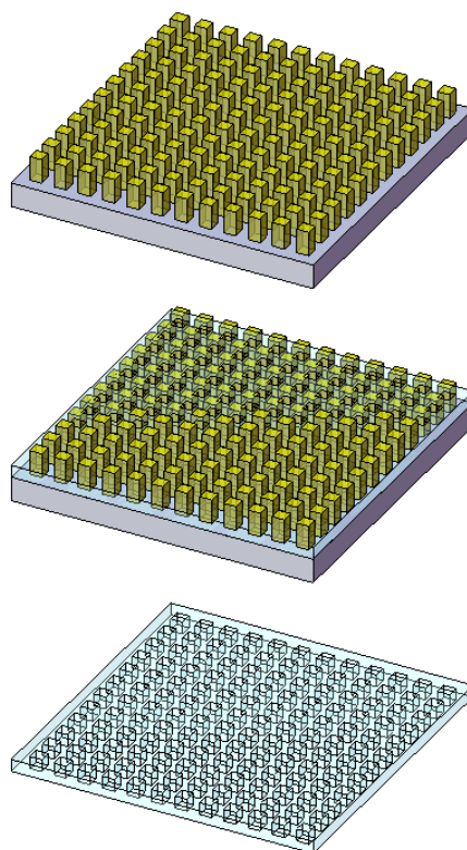
Fig. S1 – Fabrication process of PDMS grid from casting on SU-8 pillars from mold master.
