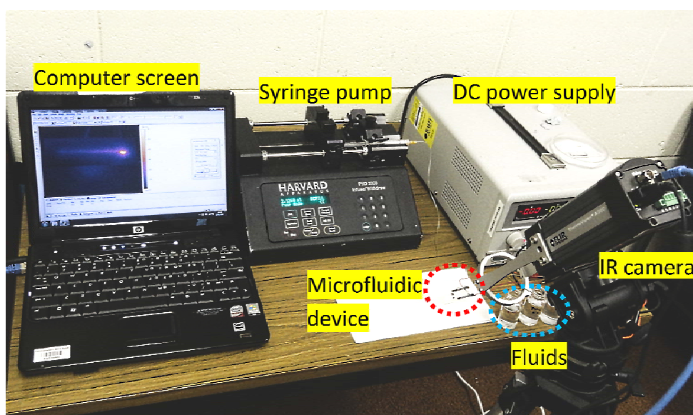
Fig. 1S. Experimental setup of our microfluidic system
