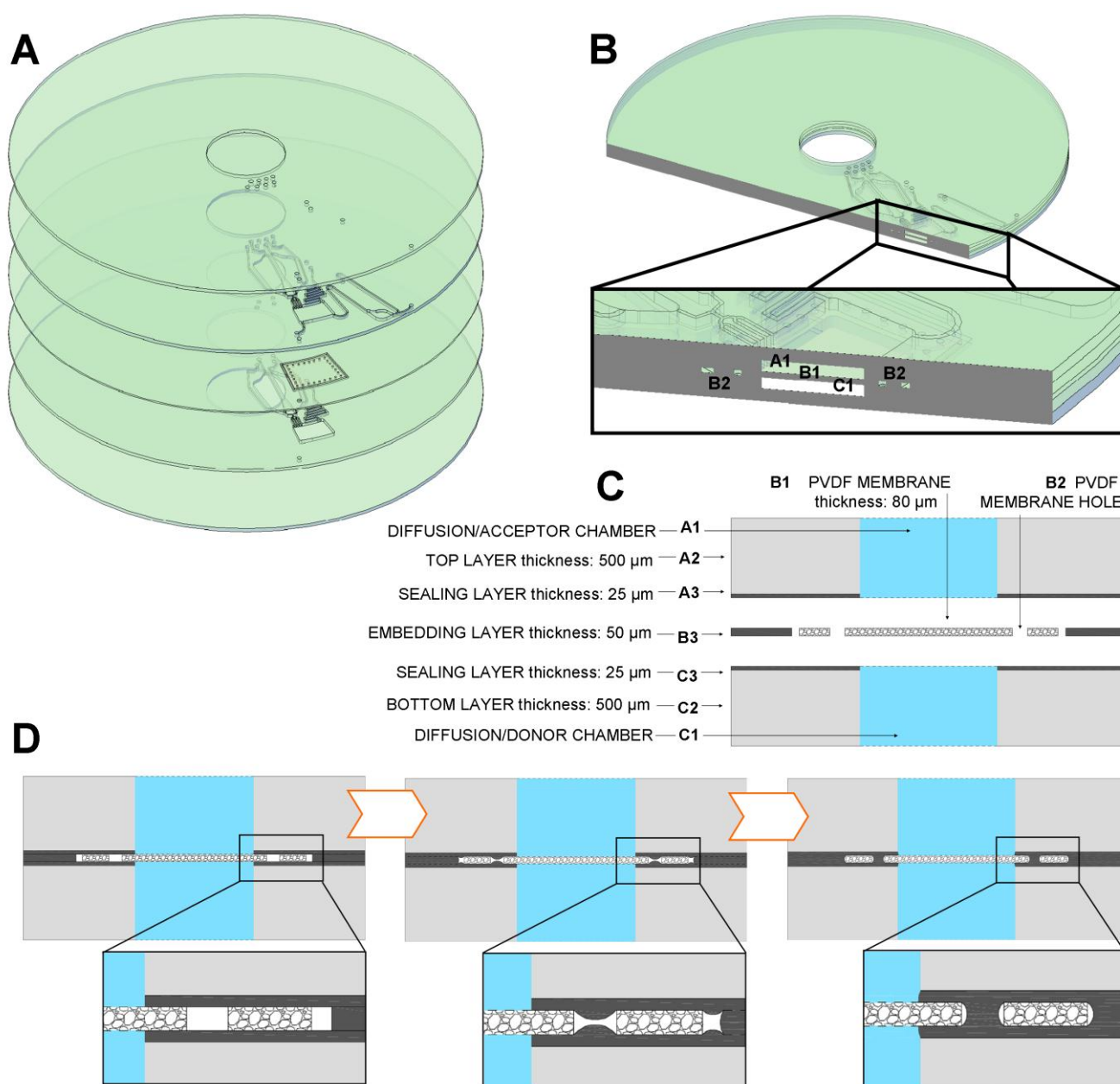
Fig. S1. A) Schematic illustration that shows the different layers of the disc. Only one of the ten microfluidic systems or subunits is represented in order to facilitate the interpretation. B) Schematic illustration of the cross section of the CD, which shows in detail the region of interest of the membrane into the diffusion chamber. C) Schematic illustration of the front view of its cross section, which shows the elements (substrate layers and membrane) involved in the membrane integration process. D) Steps of the membrane (B1) integration process during lamination, where sealing layers (A3, B3 and C3) melt into the membrane holes (B2) and ensure contact between the surrounding layers (A2 and C2).
