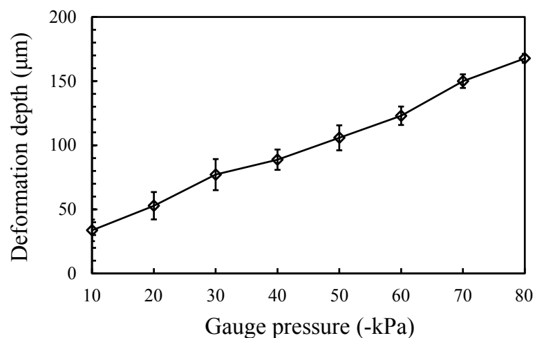
Fig. S1 The relationship between the working pressure and deformation of a PDMS membrane
