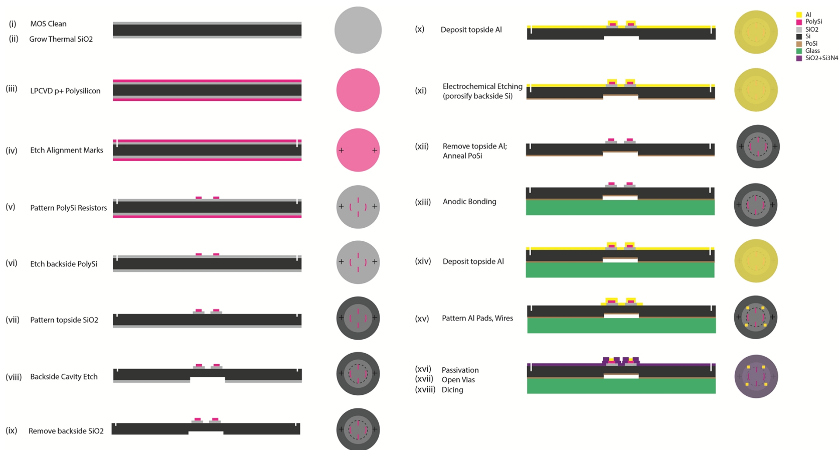
Fig. S1 Microtensimeter fabrication process flow (full). Wafer cross-sectional view (left side), top view (right side).
