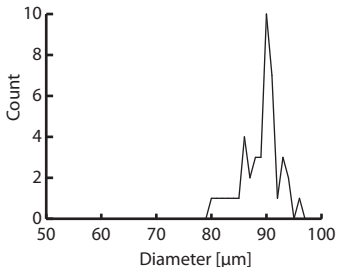
Supplementary Figure 1: Graphical representation of droplet size distribution for the 3D nozzle. The average droplet size was measured to be 89.45 \pm 3.51 \mu\text{m} .
