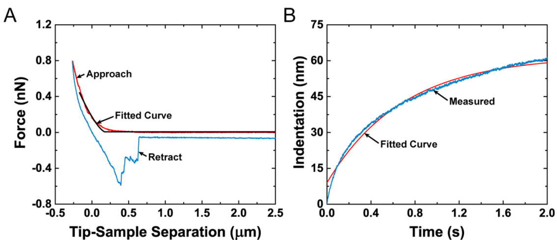
Figure S2. Overview of the atomic force microscopy mechanical property measurements. (A) Raw data of the force-indentation curve depicting the elastic deformation region. (B) Raw data of the indentation-time curve depicting the curve fit for the data set with fitted curve.
