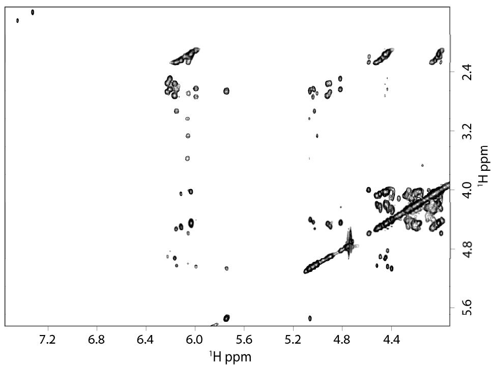
Expanded region of 2D TOCSY (700 MHz, T = 25°C) of QS55 .
