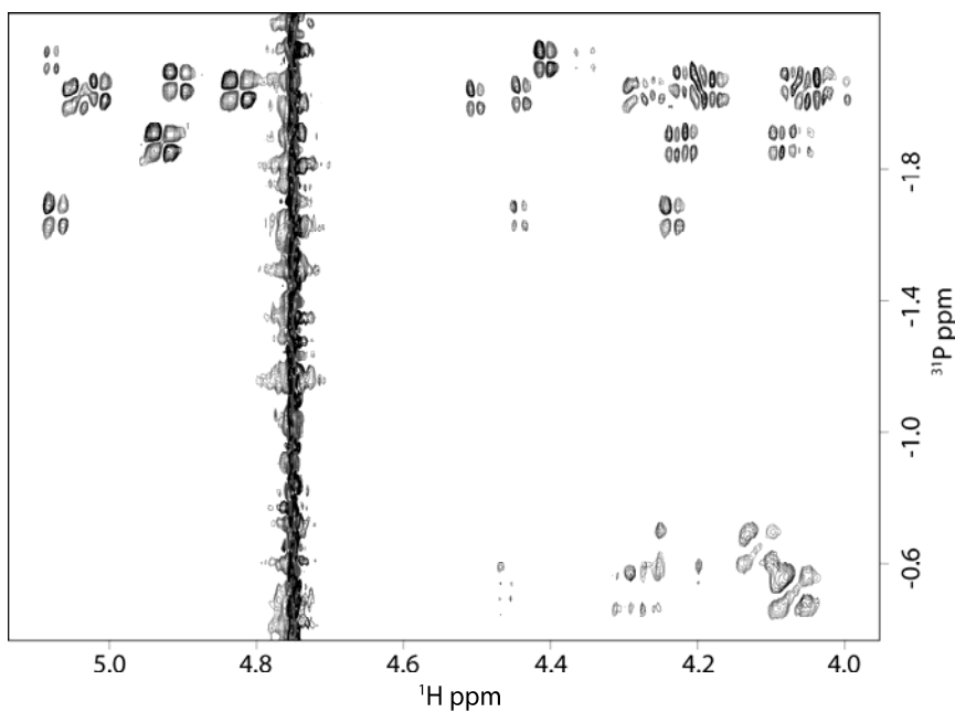
Expanded region of 2D ^{31}\text{P} - ^1\text{H} COSY (700 MHz, T = 25°C) of QS55 .
