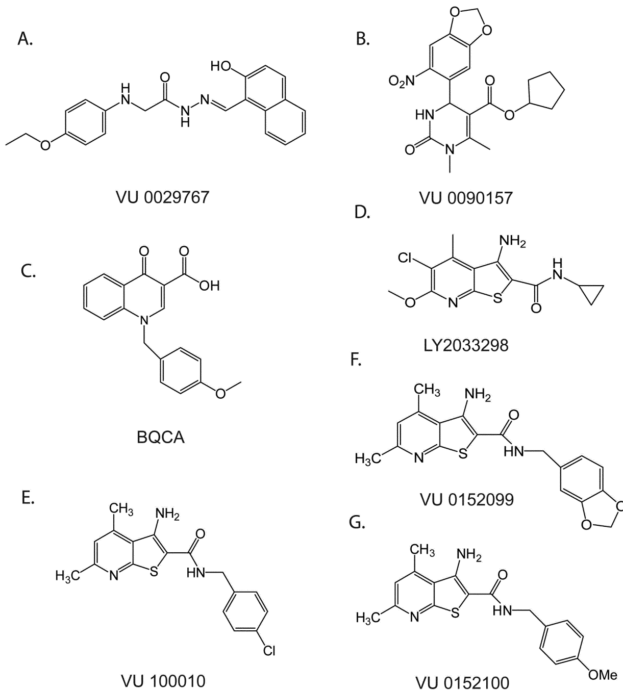
Supplemental Figure 2. Chemical structures of muscarinic positive allosteric modulators.
