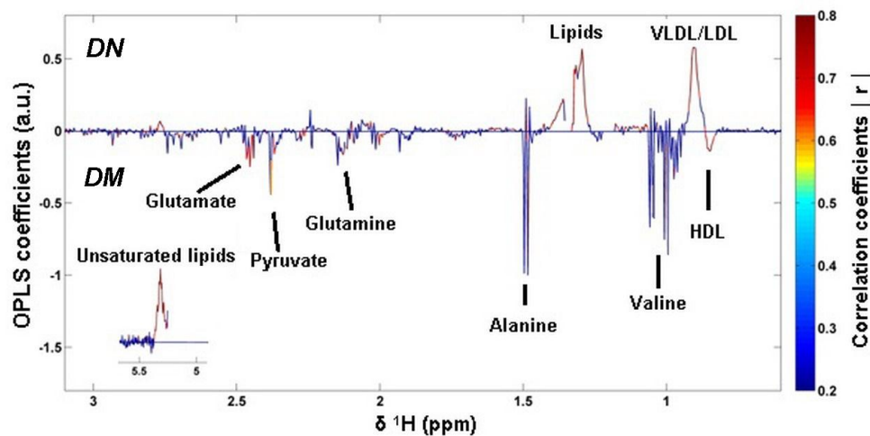
Fig. S1 OPLS-DA loading plots derived from serum 1 H NMR spectra in DN related to DM group. The colored correlation coefficients indicated significant changed metabolites which contributed to the group differentiation.
