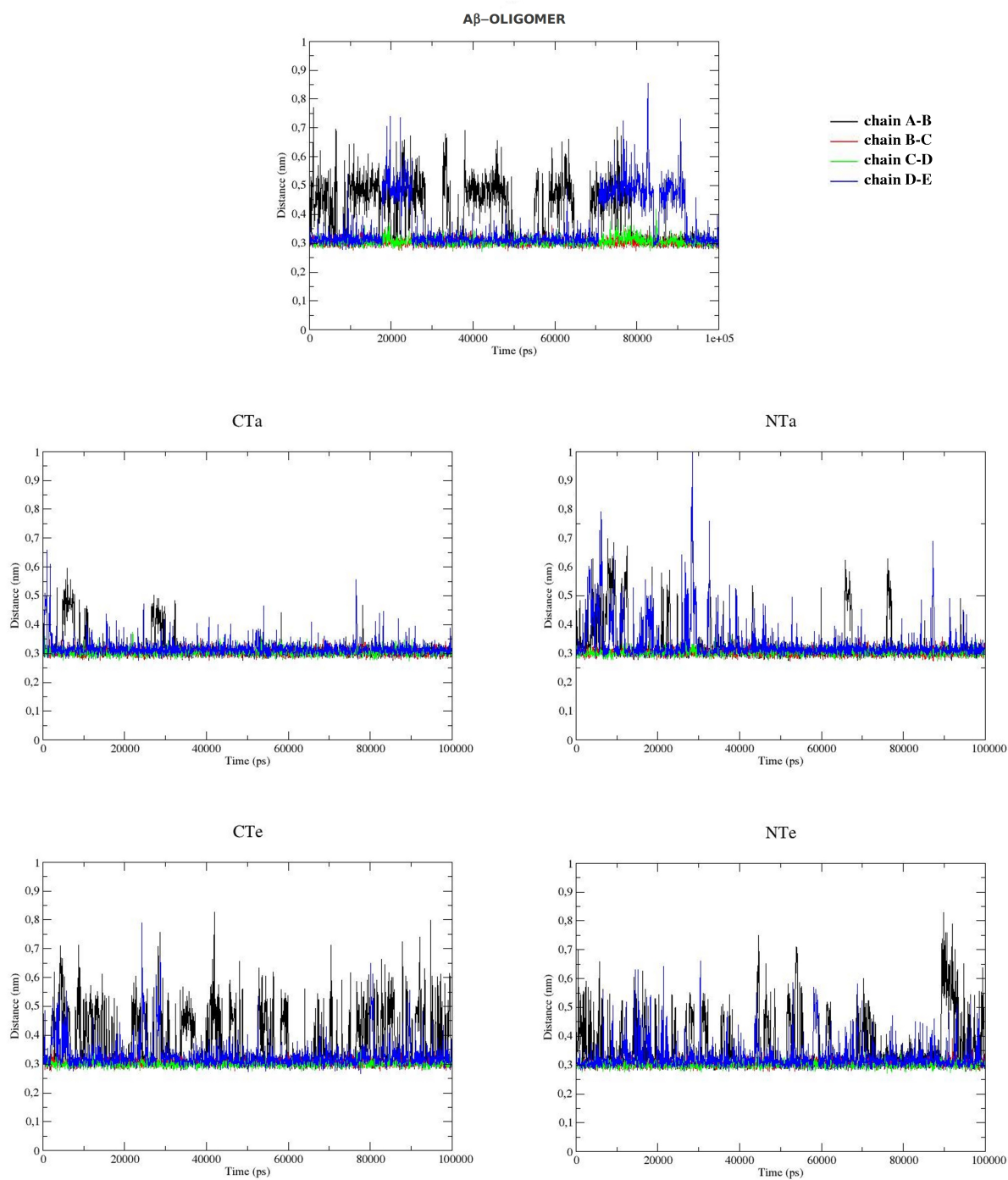
Figure S3: D23-K28 distances as a function of time for the all the systems.
