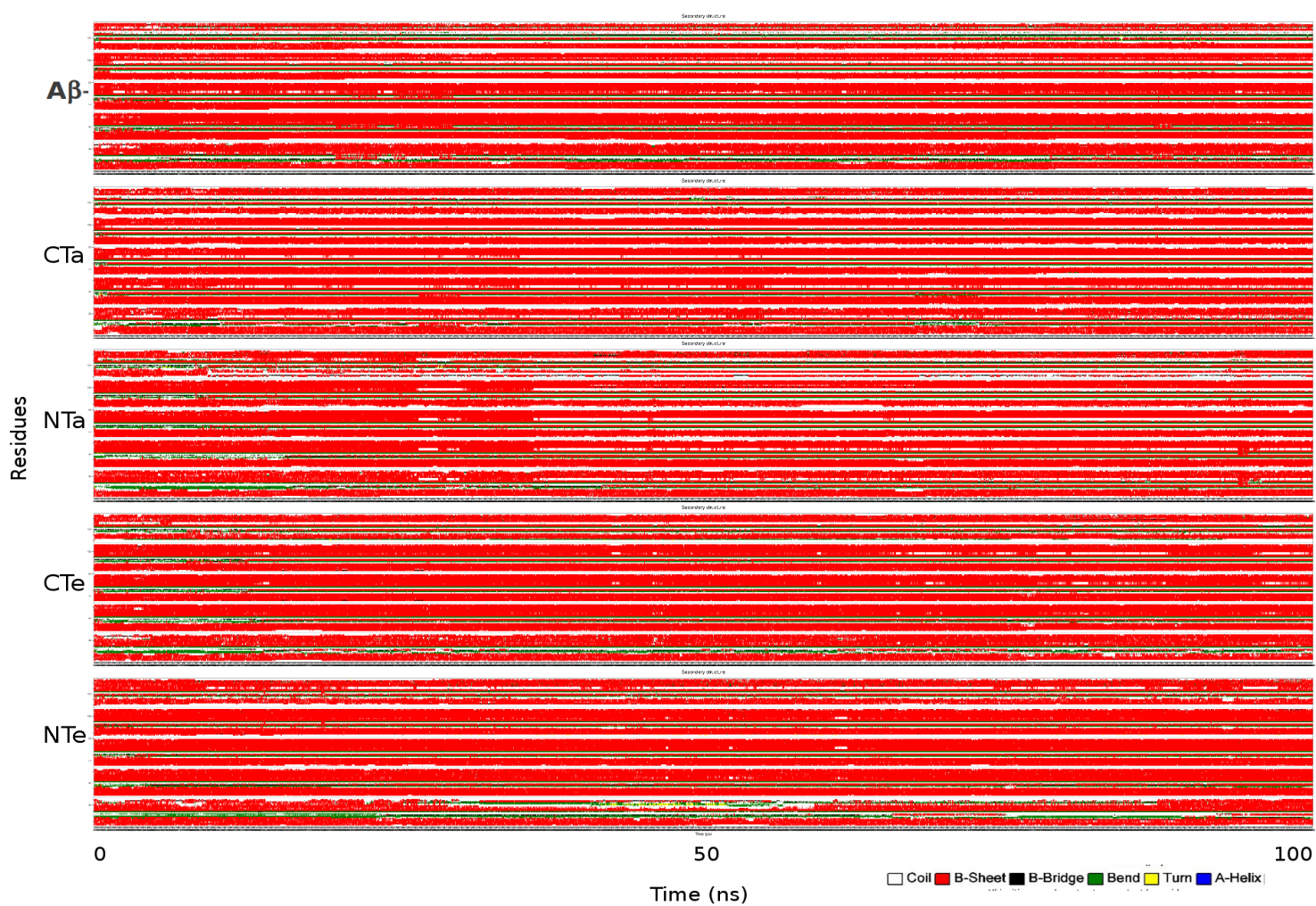
Figure S2: Secondary structures as function of time for each systems, indicated by the labels, as calculated by DSSP.
