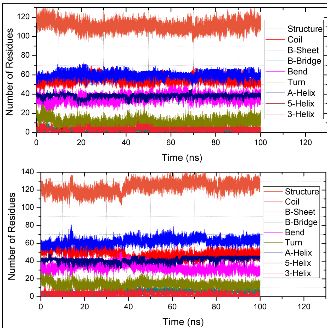
Figure S1: The secondary structure of TNKS1/2 complexes over the course of simulation. It includes the coil, \beta -sheet, \beta -bridge, bend, turn, \alpha -helix, 5-helix and 3-helix (indicated in different colors).
