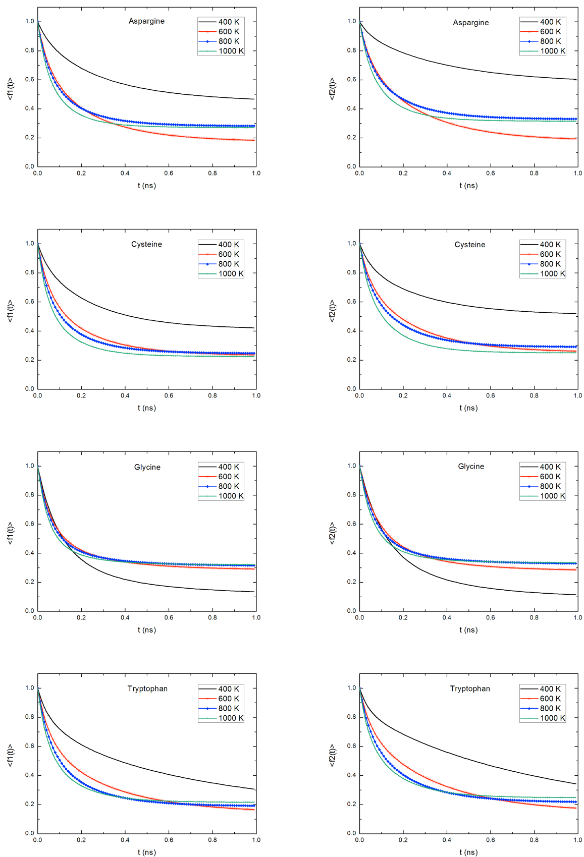
Figure S1. The mean dynamic properties \langle f_1(t) \rangle and \langle f_2(t) \rangle for Asn, Cys, Gly, Trp at 400, 600, 800 and 1000 Kelvin.
