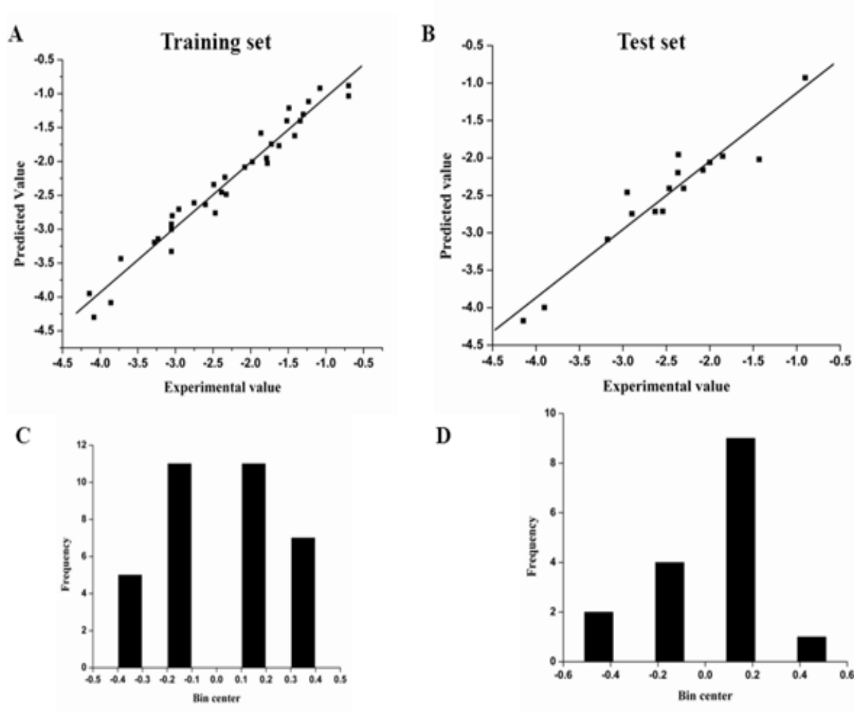
Figure S1: Correlation between predicted and experimental biological activity obtained by using the final structure-activity model for training (A) and test (B) set compounds. Residual histogram frequency statistics are shown for training (C) and test (D) set compounds.
