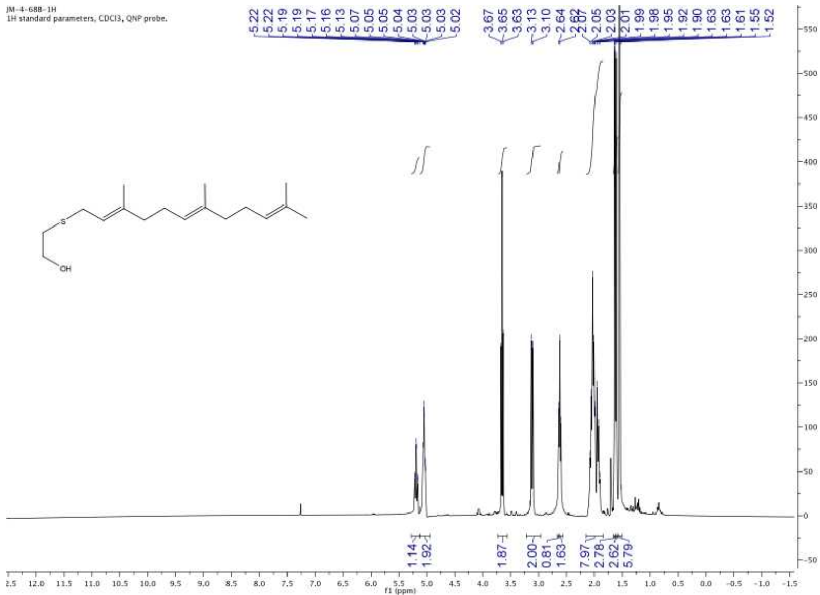
Figure A1: Proton NMR for compound 12
