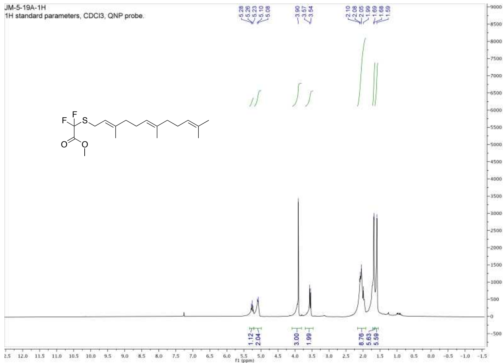
Figure A19: Proton NMR for compound 28
