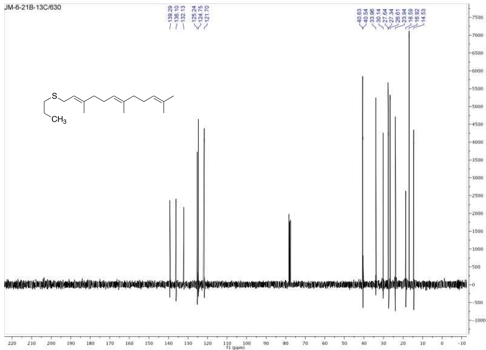
Figure A8: Carbon NMR for compound 20b
