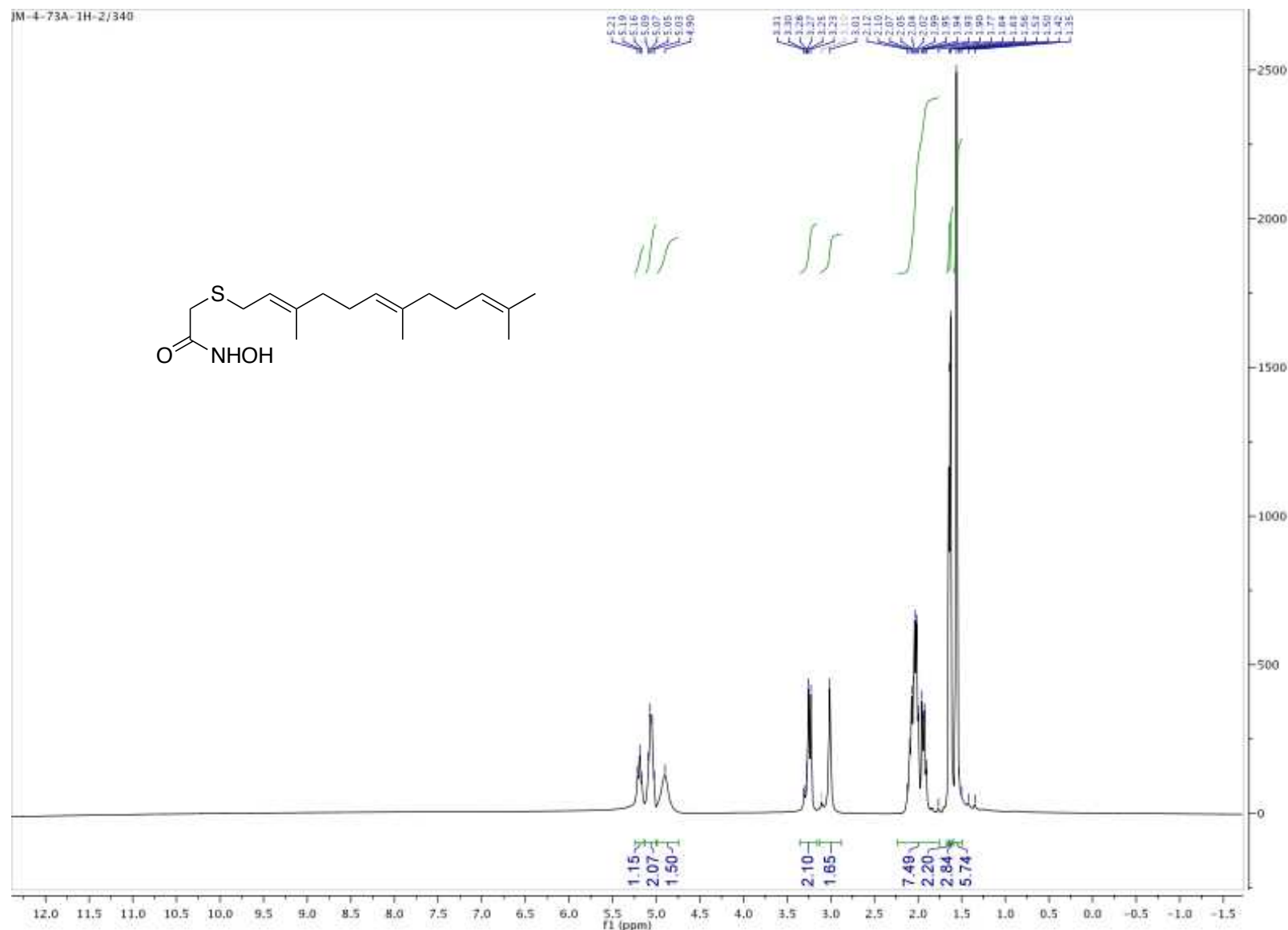
Figure A3: Proton NMR for compound 13
