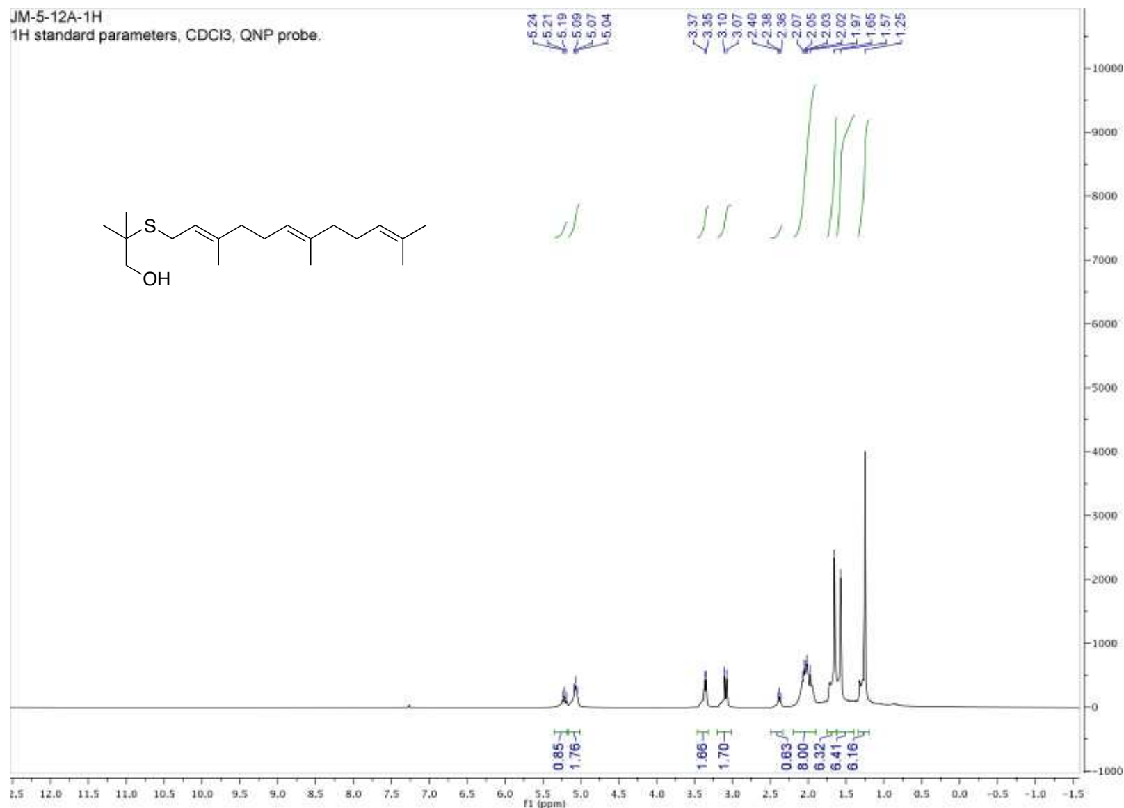
Figure A17: Proton NMR for compound 23
