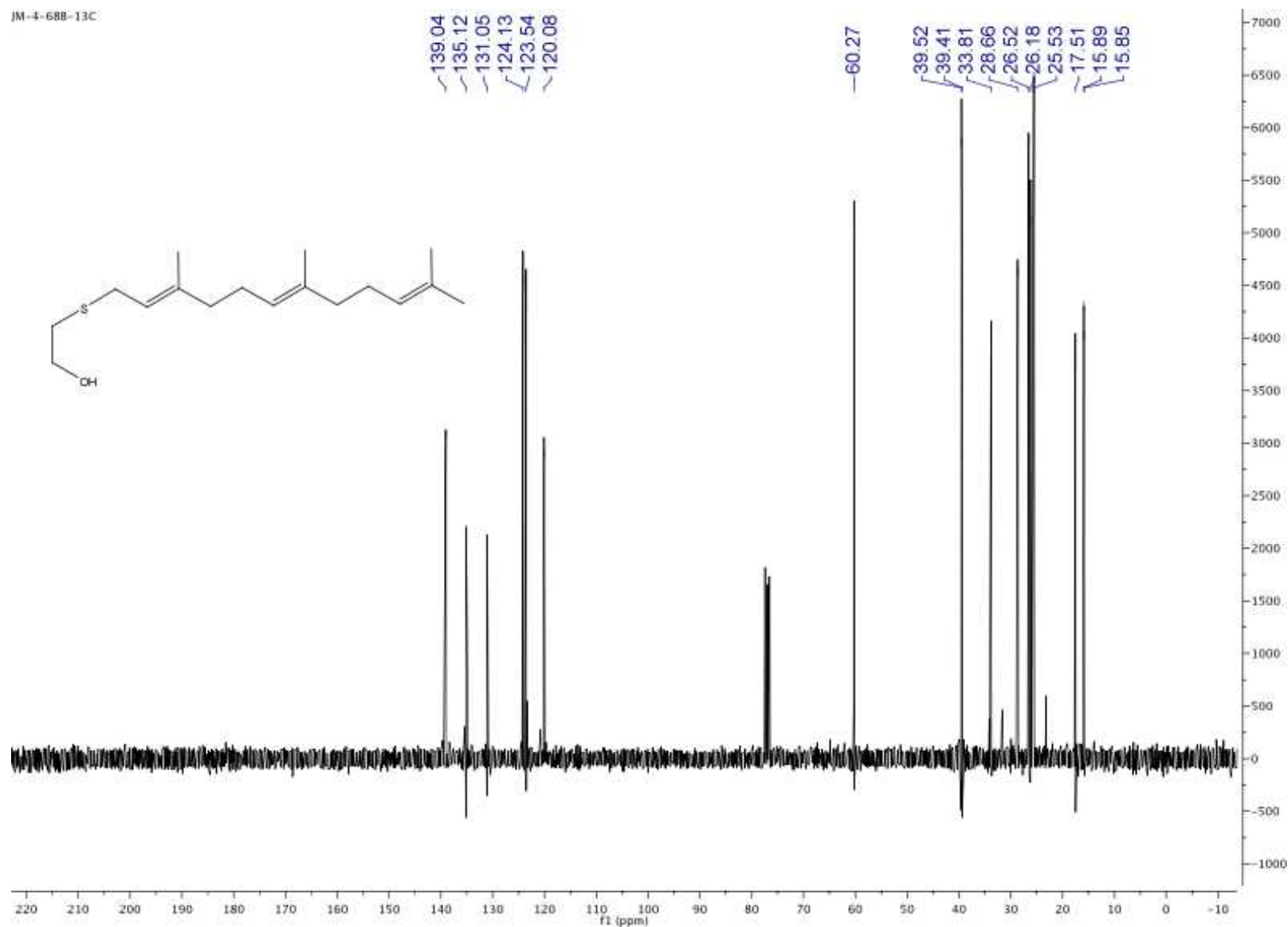
Figure A2: Carbon NMR for compound 12
