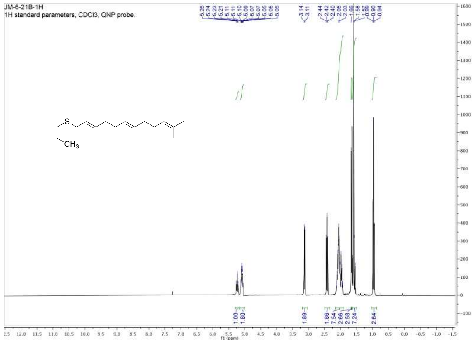
Figure A7: Proton NMR for compound 20b
