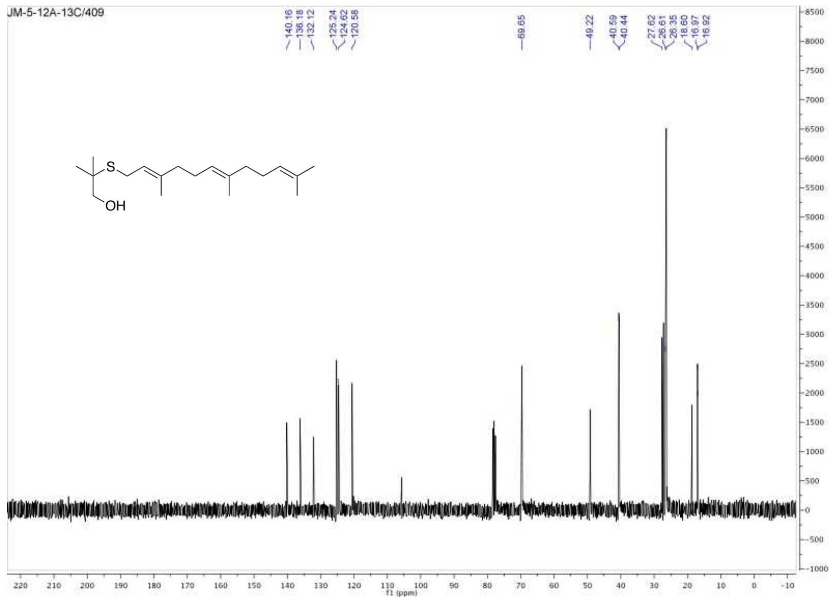
Figure A18: Carbon NMR for compound 23
