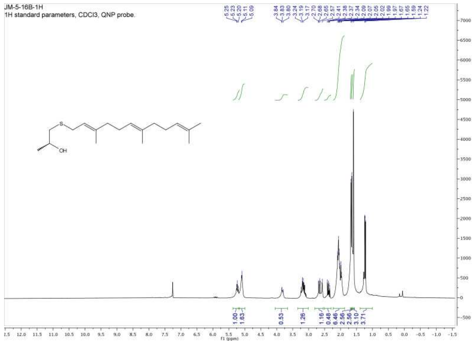
Figure A13: Proton NMR for compound 20e
