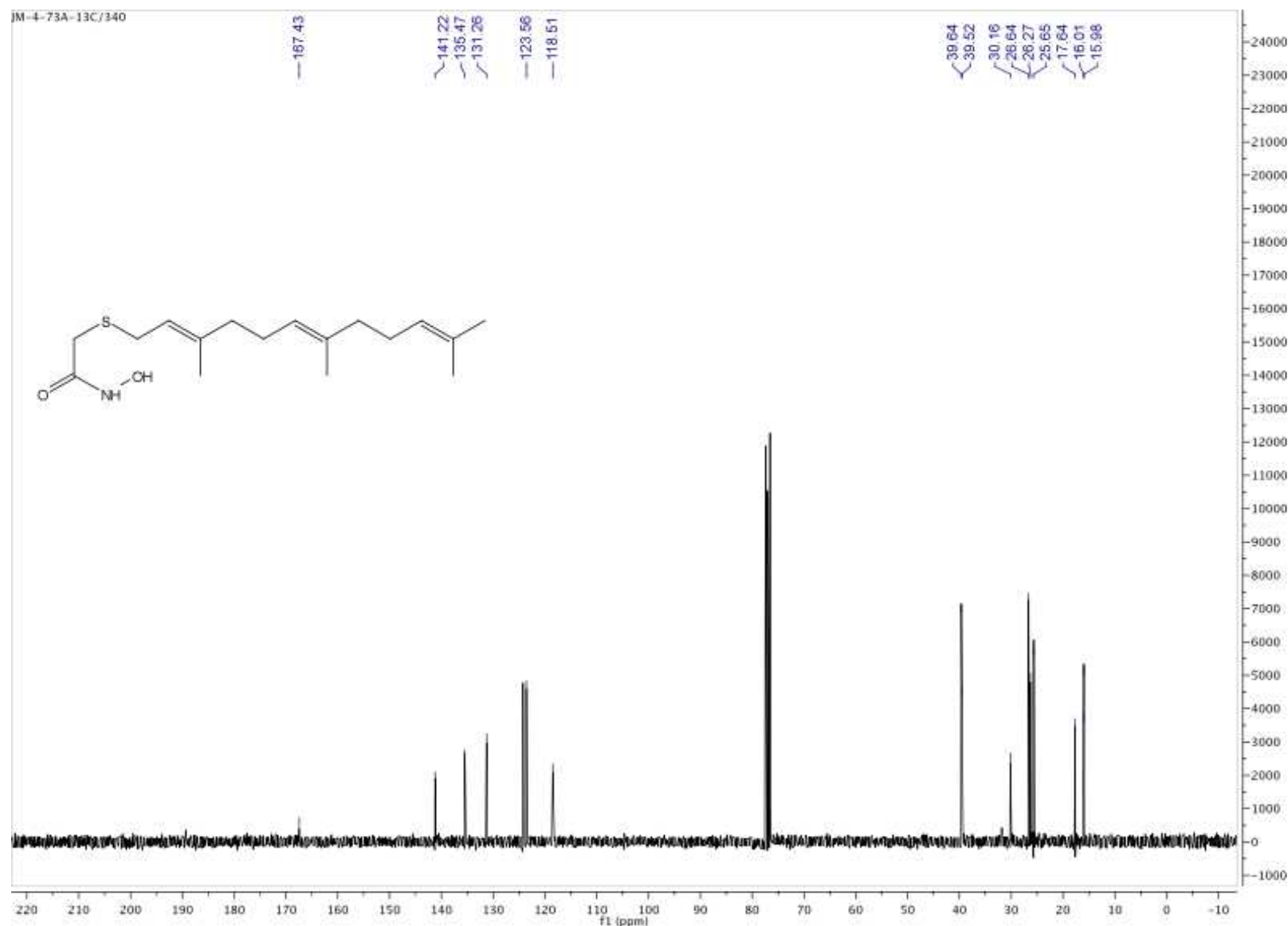
Figure A4: Carbon NMR for compound 13
