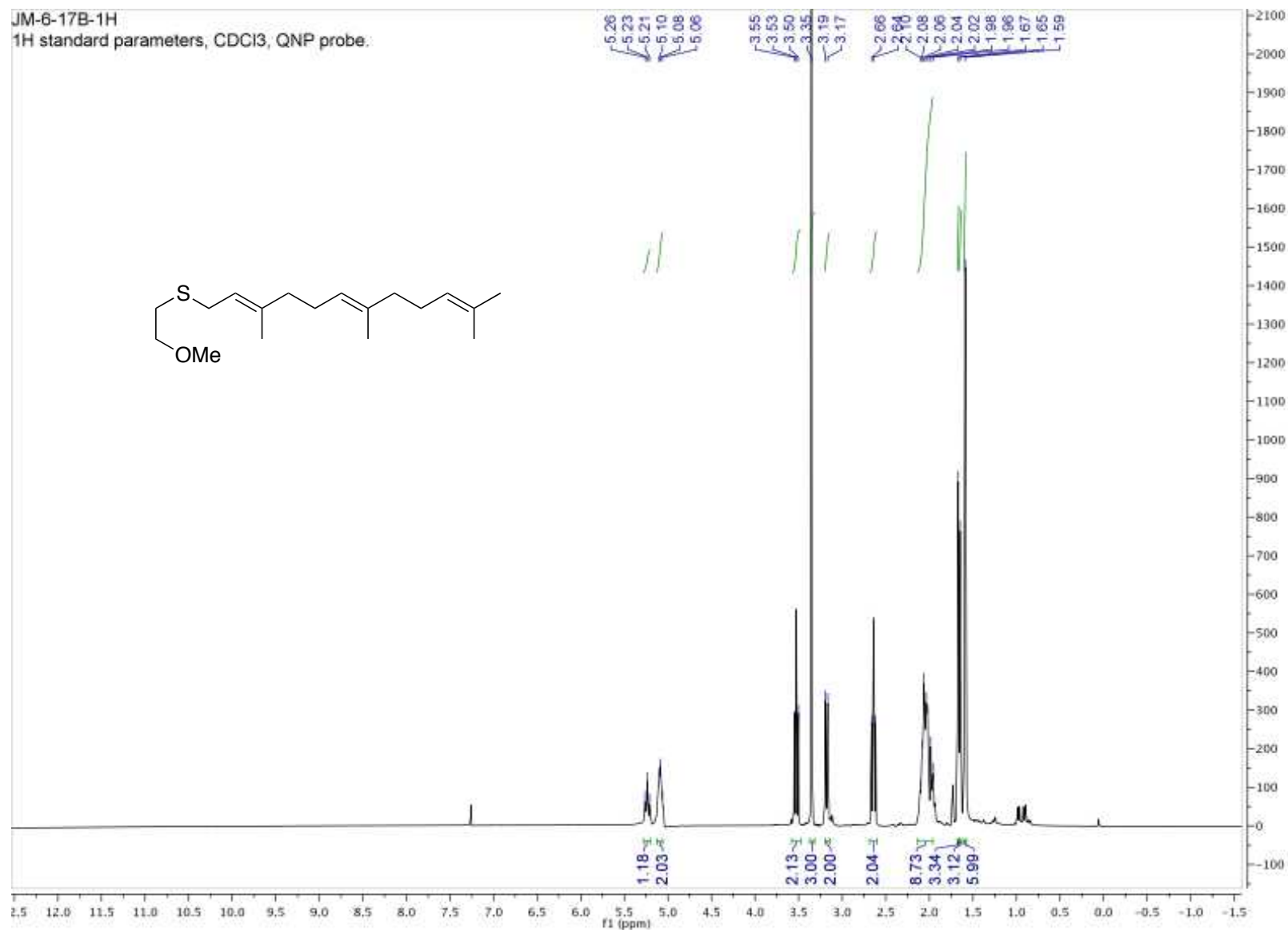
Figure A11: Proton NMR for compound 20d
