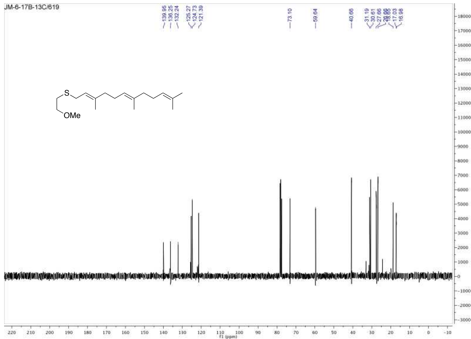
Figure A12: Carbon NMR for compound 20d
