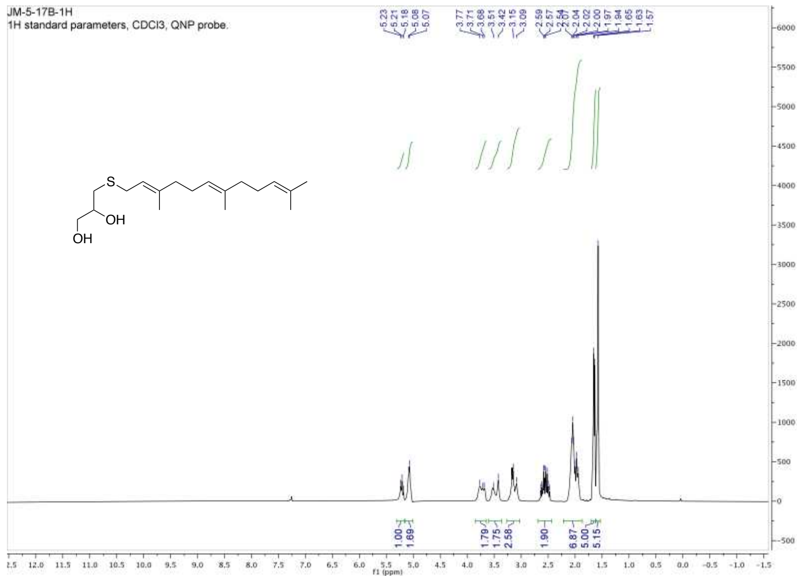
Figure A15: Proton NMR for compound 20f
