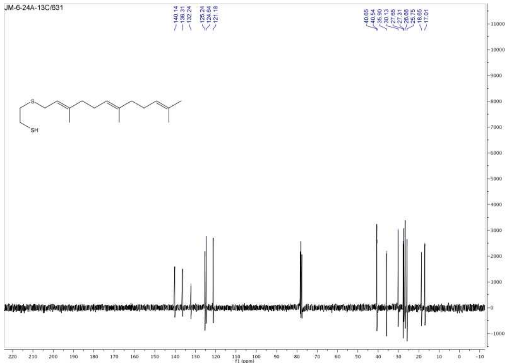
Figure A10: Carbon NMR for compound 20c
