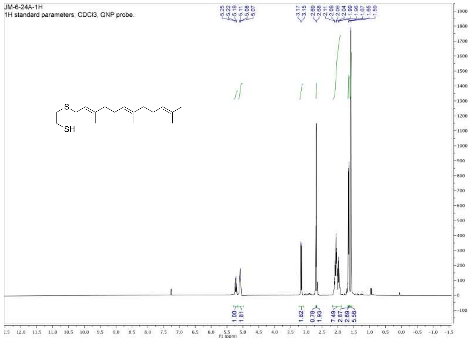
Figure A9: Proton NMR for compound 20c
