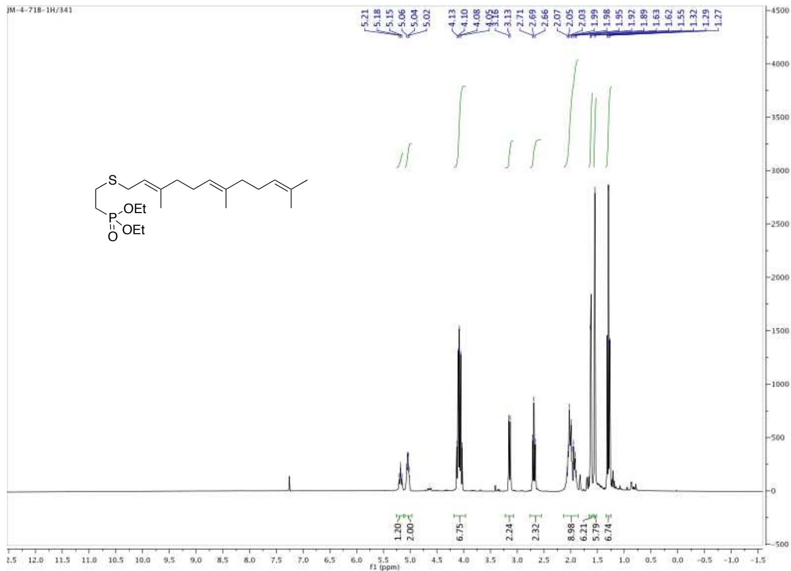
Figure A5: Proton NMR for compound 17
