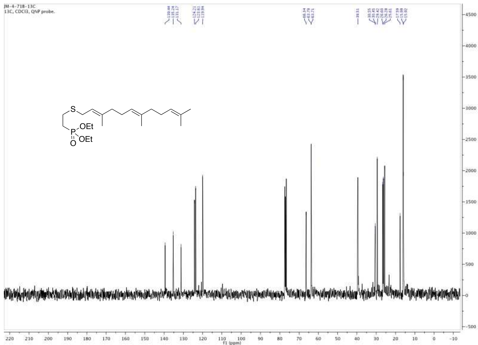
Figure A6: Carbon NMR for compound 17
