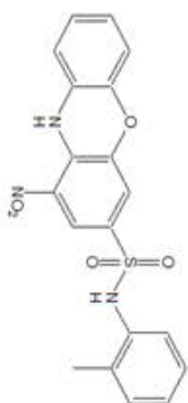
1 H-NMR of compound 6o
