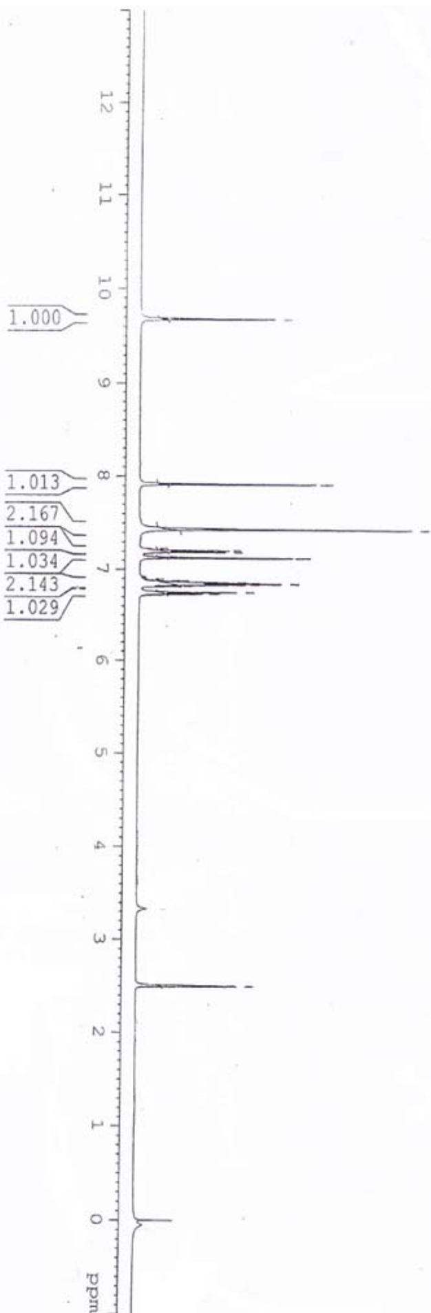
1 H-NMR of compound 6a
