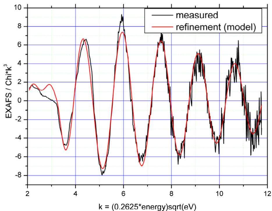
Zn-K-edge EXAFS of Zn(II)-glutathione pH7
