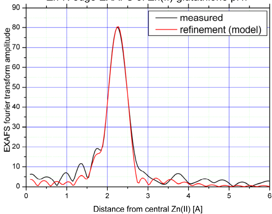
Zn-K-edge EXAFS of Zn(II)-glutathione pH7
