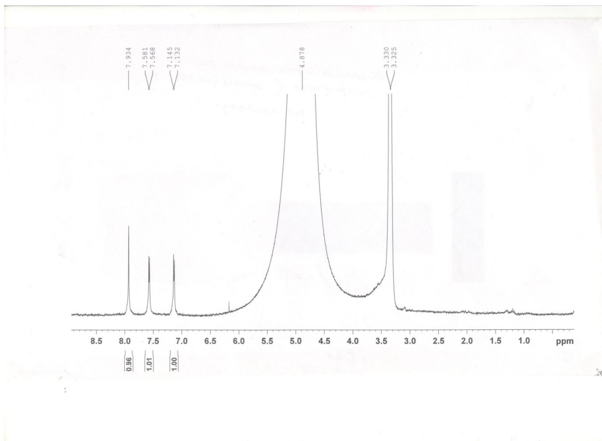
Fig.5 1 H NMR spectra of 5-nitrofurfural-2-thiosemicarbazone
