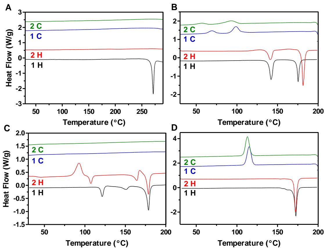
Fig. S2 DSC thermograms of A) Pt-3C, B) Pt-5C, C) Pt-6C, and D) Pt-8C obtained in nitrogen at heating and cooling rates of 10 °C/min.
