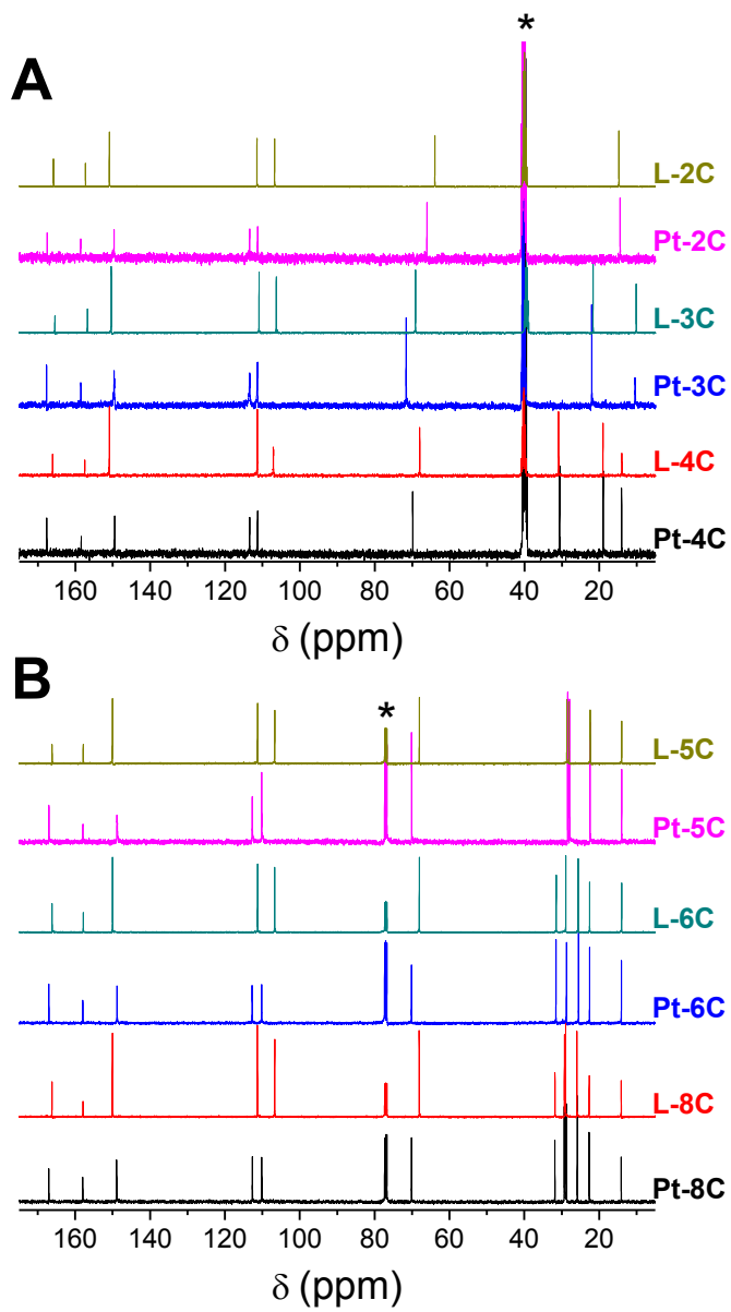
Fig. S1 ^{13}\text{C} NMR spectra of ligands and Pt(II)-complexes recorded in A) \text{DMSO-}d_6 and B) \text{CDCl}_3 at temperatures indicated in the experimental section (* solvent peak).
