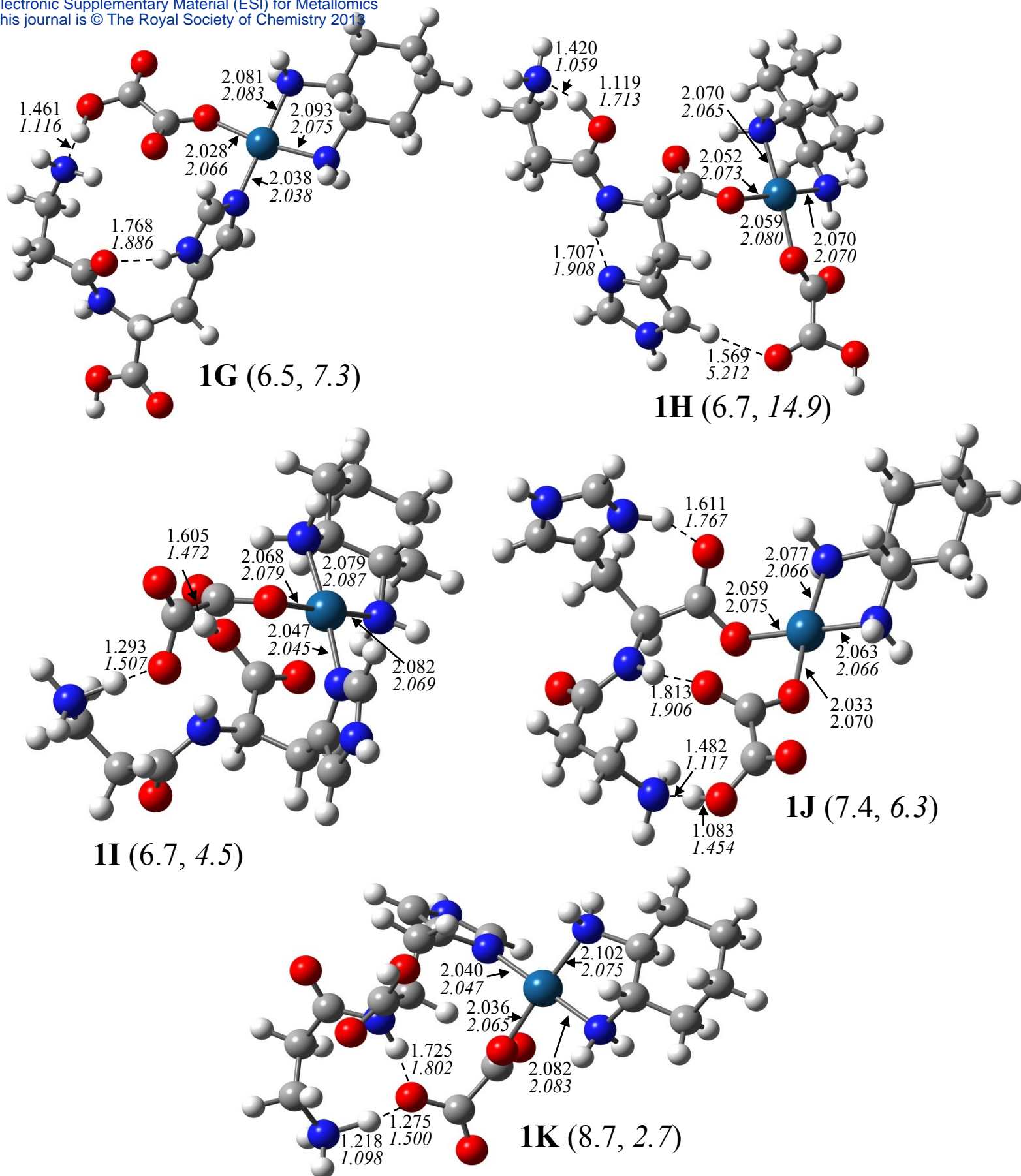
Figure S12: Structures for [\text{Carnosine} + \text{OxPt} + \text{H}]^+ ions in which a formal Pt coordination to carnosine is observed as calculated at the B3LYP/LANL2DZ level of theory. Bond lengths are in Angstroms, relative free energies are indicated in parenthesis. Italicized numbers are for solvated species.
