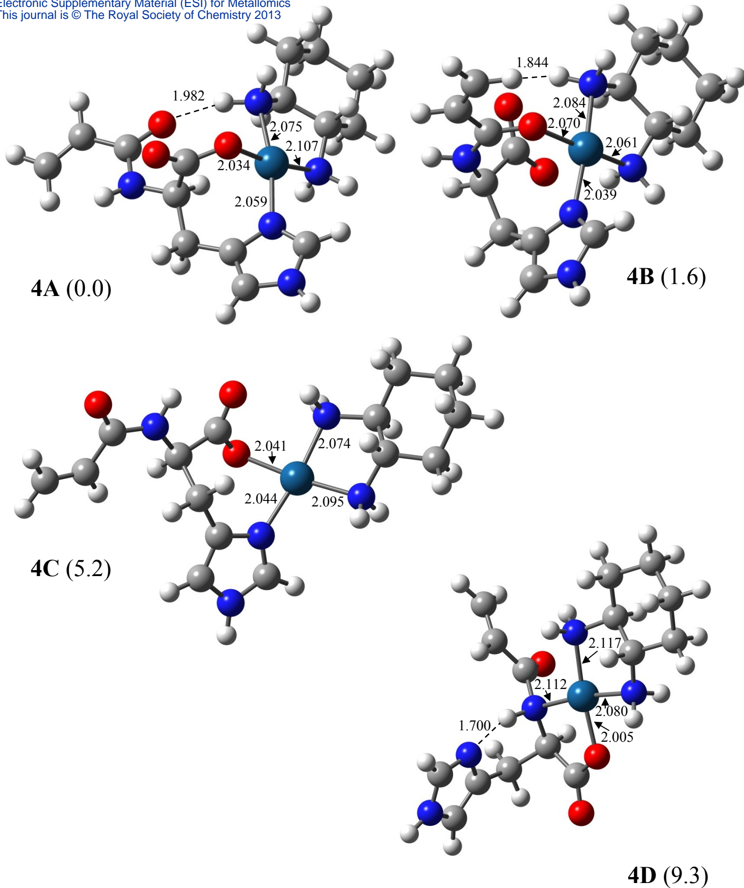
Figure S14: Structures for [\text{Carnosine} - \text{NH}_3 - \text{H} + \text{Pt}(\text{dach})]^+ ions as calculated at the B3LYP/LANL2DZ level of theory. Bond lengths are in Angstroms, relative free energies are indicated in parenthesis.
