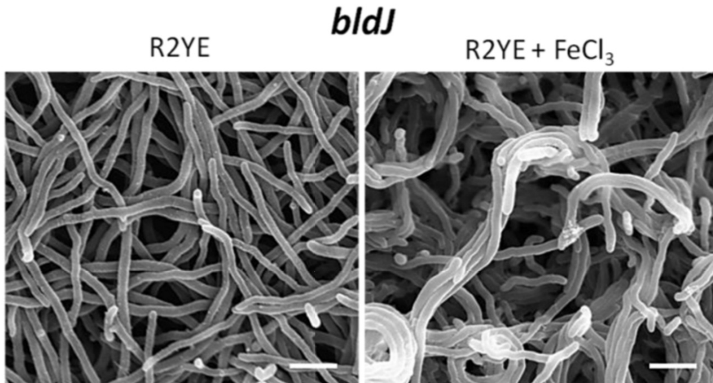
Fig. S2. Effect of FeCl 3 on development of the bldJ mutant after five days of growth. Note that the sporulation is not fully restored and that many of the aerial hyphae are stuck one to each other.
