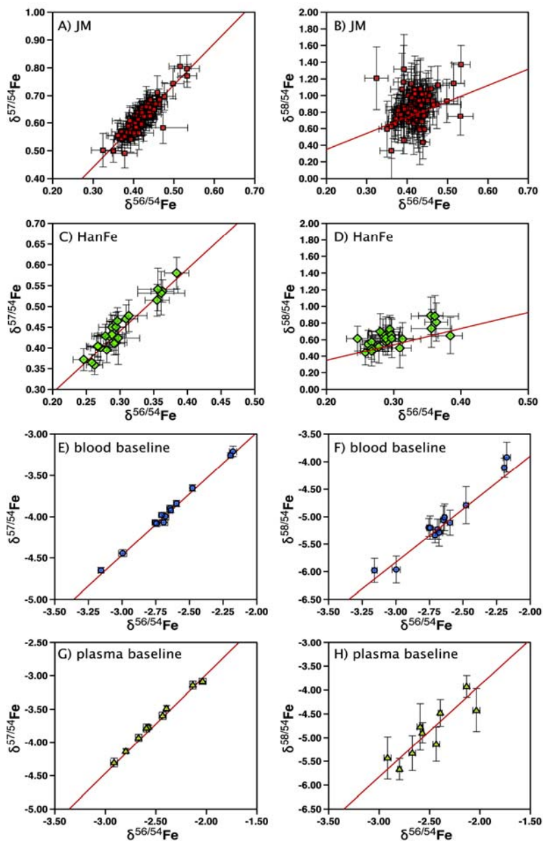
Figure S1: \delta^{57}\text{Fe} versus \delta^{56}\text{Fe} and \delta^{58}\text{Fe} versus \delta^{56}\text{Fe} , respectively, of internal standard materials "JM" (a) and (b); of internal standard material "HanFe" (c) and (d); of baseline blood samples (e) and (f); of baseline plasma samples (g) and (h).
