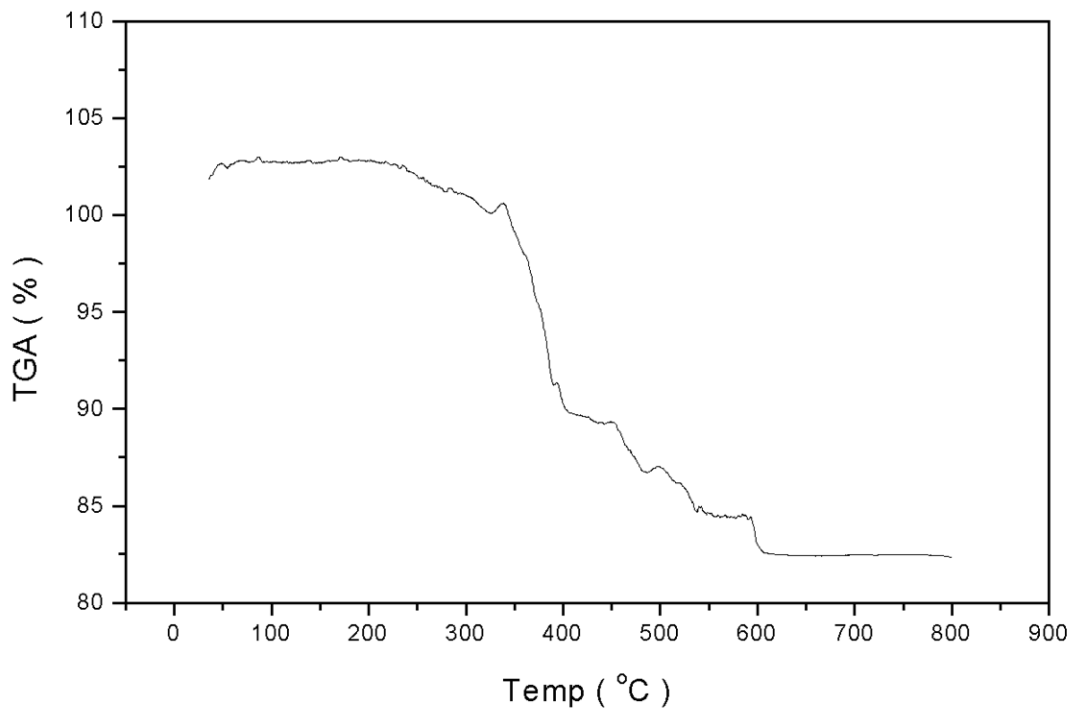
TGA diagram of ZCP-THO
