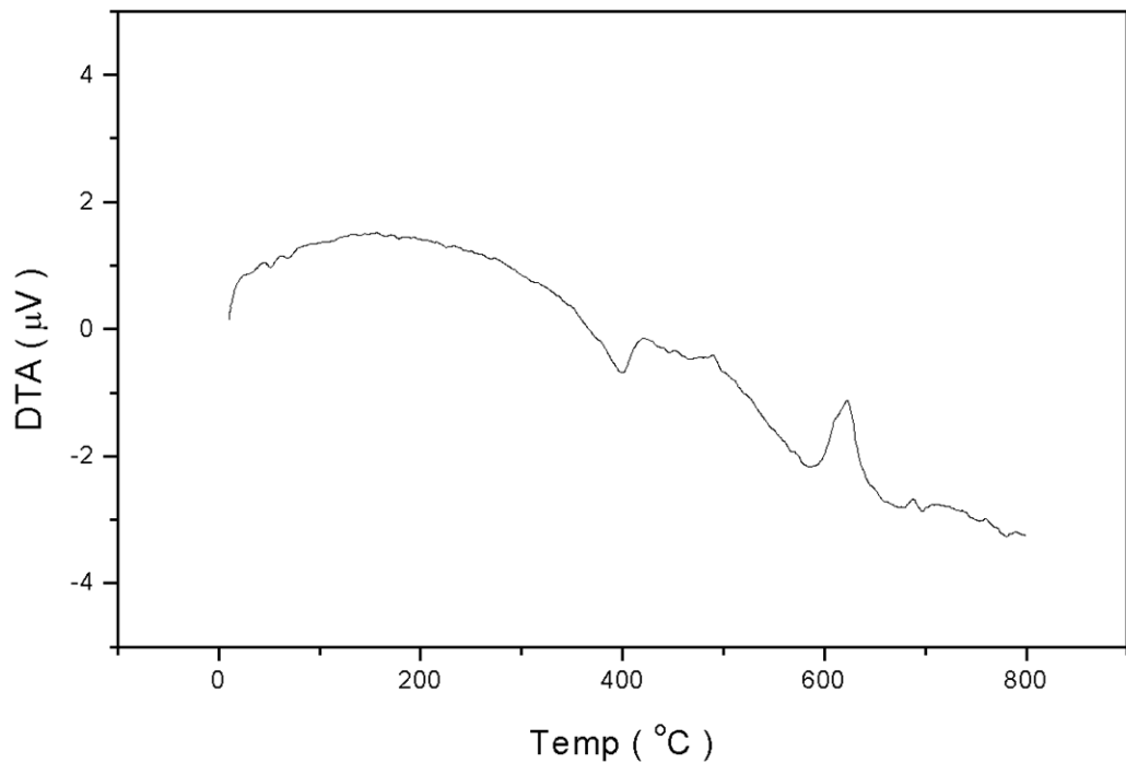
DTA diagram of ZCP-THO
