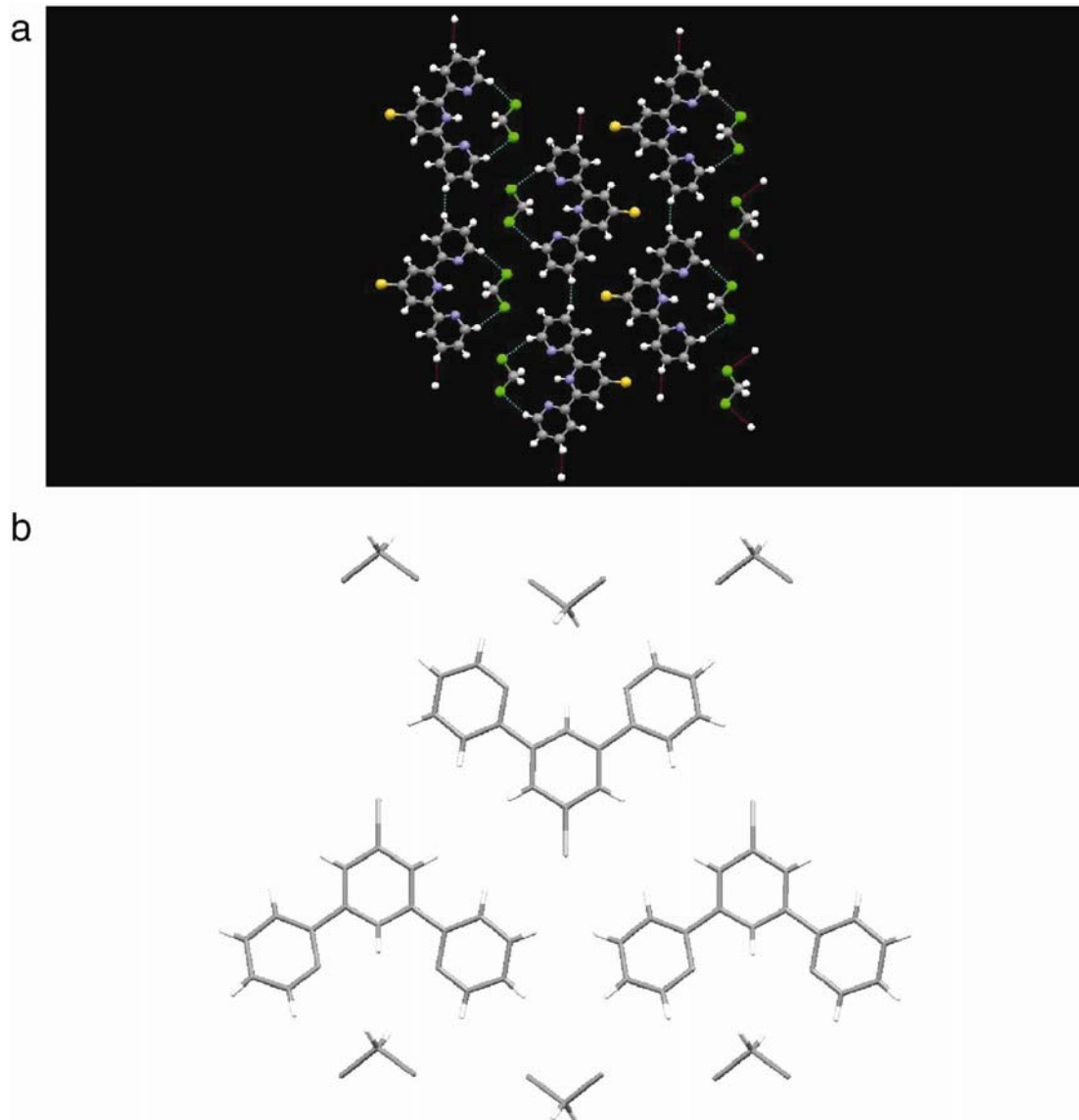
Figure 2 Sheets are formed containing {1.CH 2 Cl 2 } units linked by non-classical C-H...X interactions to both the solvent molecule and the sulfur of another molecule of 1.
