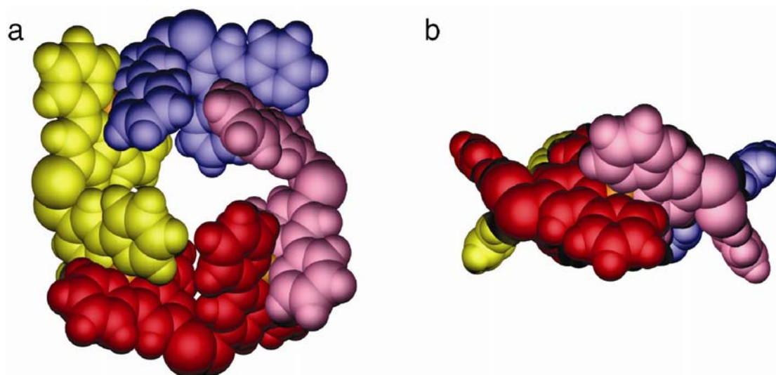
Figure 6 Space-filling representations of the metallomacrocyclic [\text{Fe}_4(2)_4]^{8+} cation in [\text{Fe}_4(2)_4][\text{BF}_4]_8 from (a) above and (b) the side. The individual ligands have been coloured to assist the viewer.
