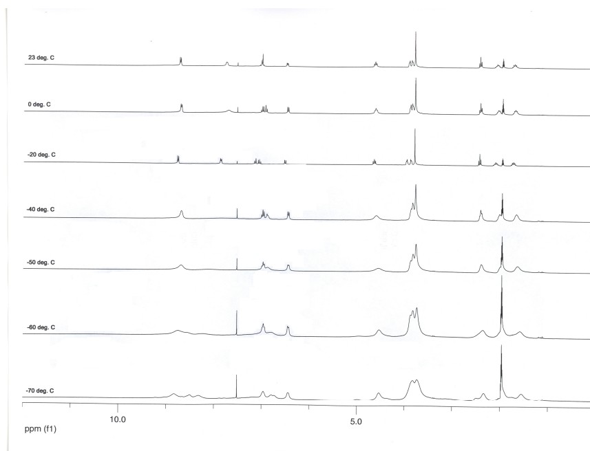
Fig. S1: Variable-temperature 1 H-NMR spectra for 4·2PF 6 /BN-38-C-10
