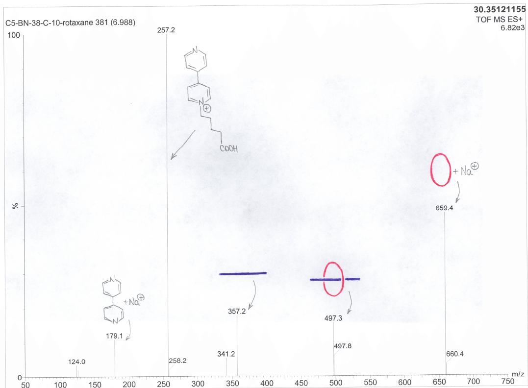
Fig. S2: ESI-MS spectrum for 4·2PF 6 /BN-38-C-10
