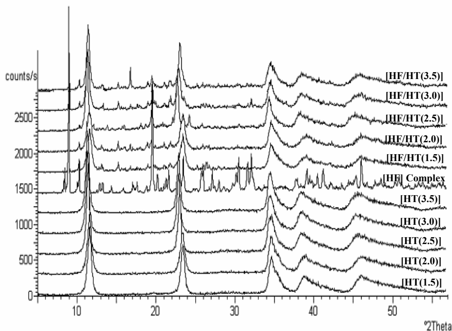
Fig. S2 P-XRD patterns of [HF] complex, [HT(3.5)] and [HF/HT(X)] system.
