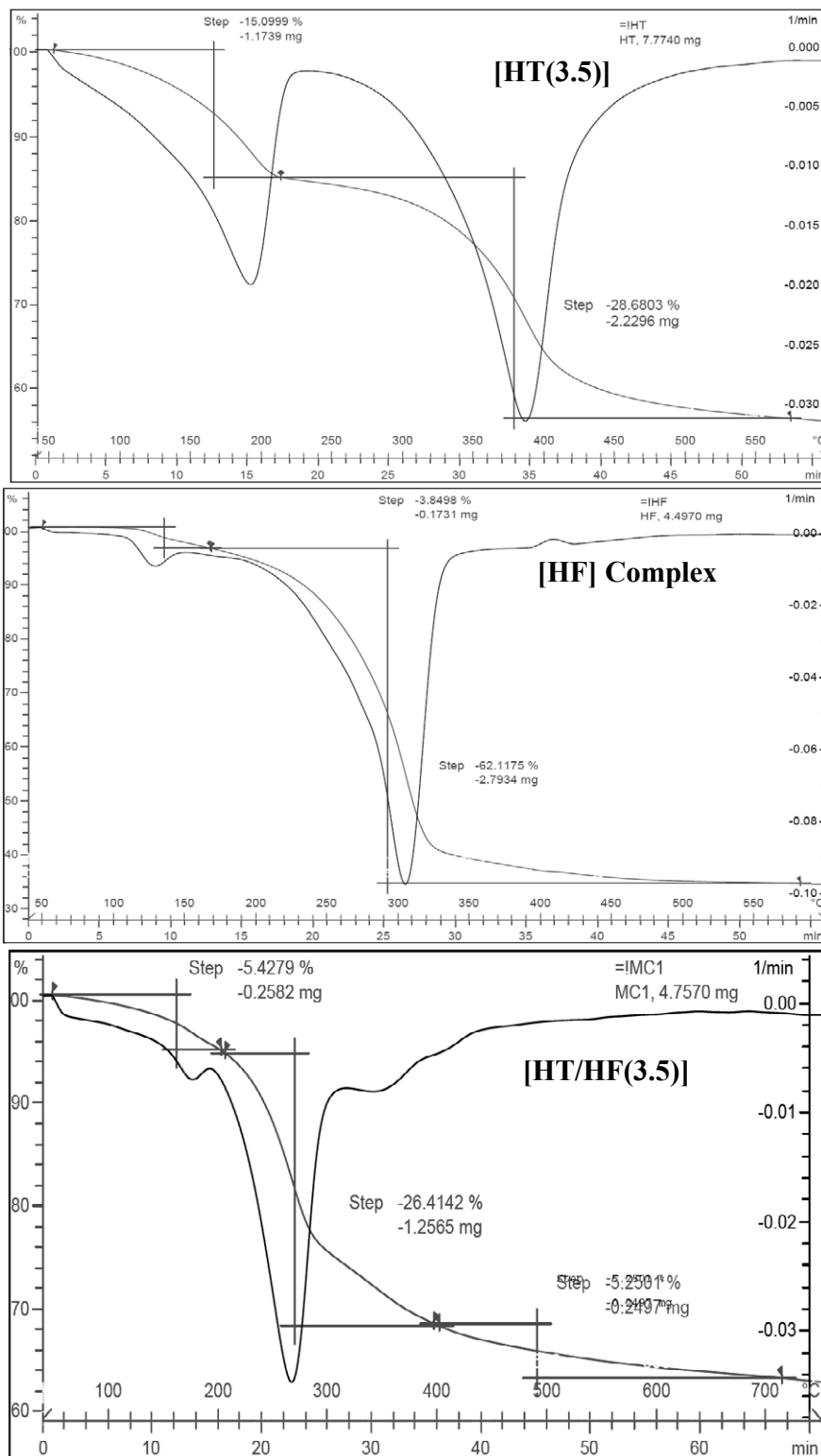
Fig. S4 TGA of [HT(3.5)], [HF] Complex and [HT/HF(3.5)].
