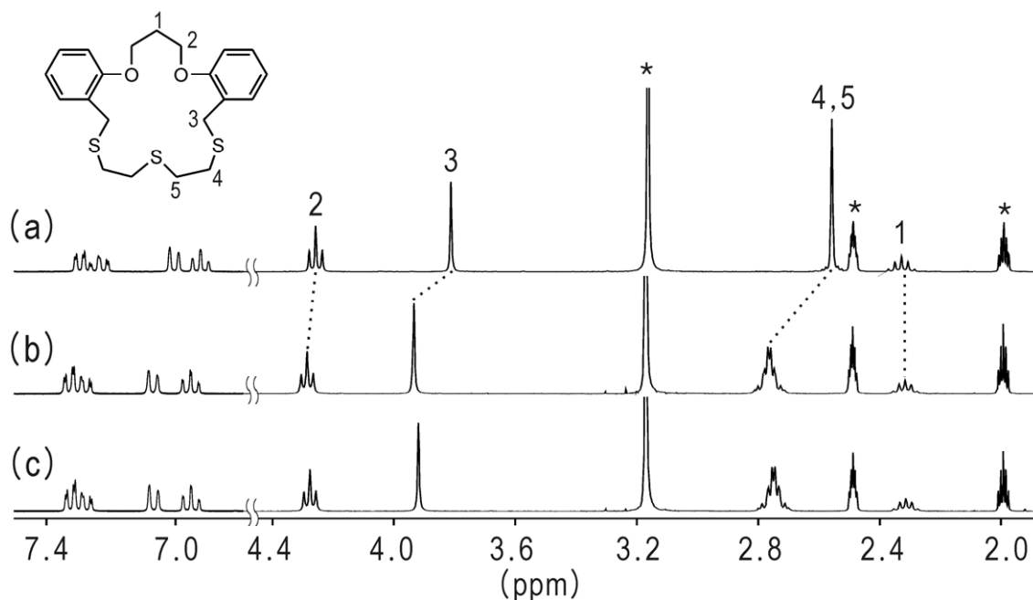
Fig. S1. 1 H-NMR spectra of (a) free L 1 , (b) L 1 + AgNO 3 (1.0 equiv.) and (c) L 1 + AgPF 6 (1.0 equiv.) in CD 3 CN:DMSO- d 6 (1:1). The peaks marked with an asterisk are from solvents and water.
