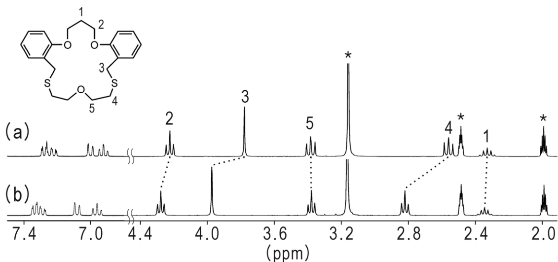
Fig. S2. 1 H-NMR spectra of (a) free L 2 and (b) L 2 + AgNO 3 (1.0 equiv.) in CD 3 CN:DMSO- d 6 (1:1). The
