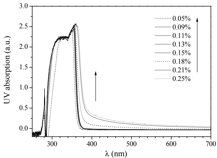
Figure S1. UV-vis spectra of 2 in toluene, at different concentrations, at 25°C.
