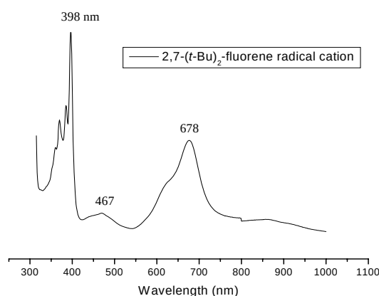
Fig. S1. UV-Visible spectrum of the 2,7-(t-Bu) 2 -F radical cation obtained along an in situ anodic oxidation of a solution of 2,7-(t-Bu) 2 -F in CH 2 Cl 2 + Bu 4 NPF 6 0.2 M at 1.6 V vs Fc/Fc + . Working platinum electrode.
