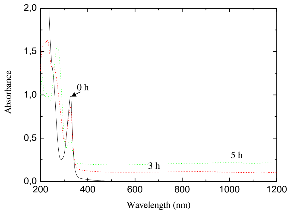
Figure S1: Absorption spectrum evolution with UV irradiation of a solution containing 10^{-3} \text{ mol L}^{-1} \text{ Pd(acac)}_2 in 2-propanol under 1 atm of CO. Optical path = 1 mm.
