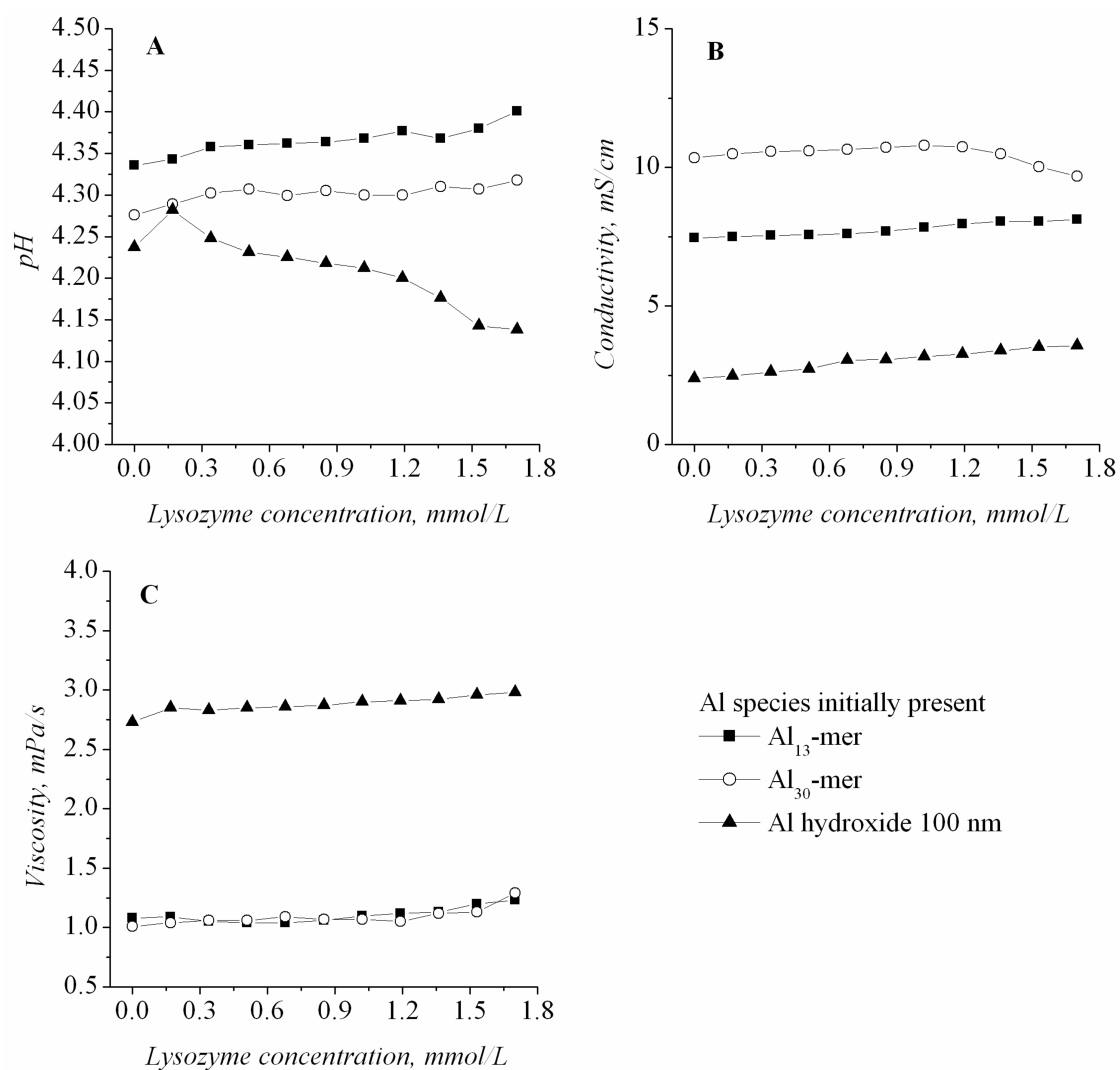
Fig. S1 (A) pH, (B) conductivity and (C) viscosity of aluminium species-lysozyme samples prepared at various protein concentrations.
