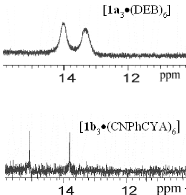
Figure SI 1 1 H NMR spectra of double rosette assemblies 1a 3 •(DEB) 6 and 1b 3 •(CNPhCYA) 6 recorded in [D] 8 -toluene at 300 MHz.
