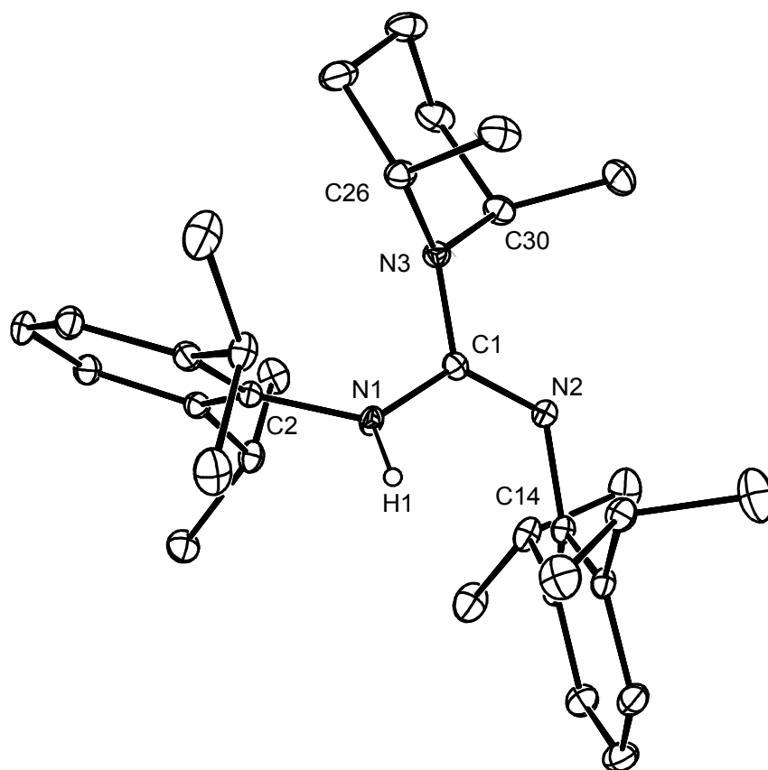
Figure S2. Molecular structure of PipisoH 3 (25% thermal ellipsoids are shown; hydrogen atoms, except H(1), omitted for sake of clarity).
