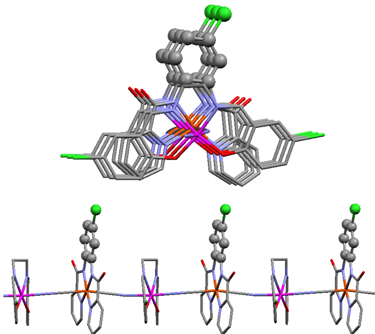
Fig. S1. Diagrams showing the arrangement of the bpClb 2- ligands in a chain of complex 1 .
