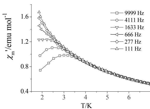
Fig. S3. Temperature dependence of in-phase ( \chi' ) ac magnetic susceptibility measured under the dc magnetic field of zero for complex 4 .
