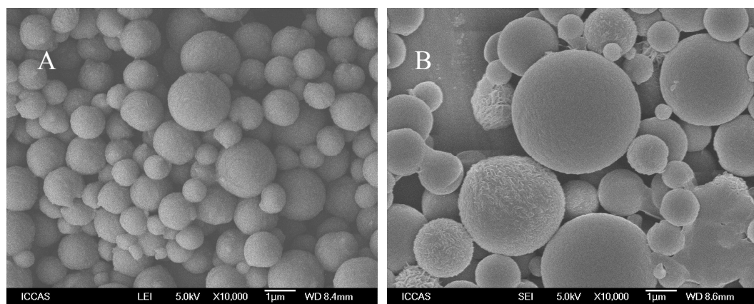
Fig. S1 SEM images of particles prepared from small molecular weight polyethylene. A: polyethylene with molecular weight of M_w=87,500 g/mol; B: polyethylene with molecular weight of M_w=121,800 g/mol.
