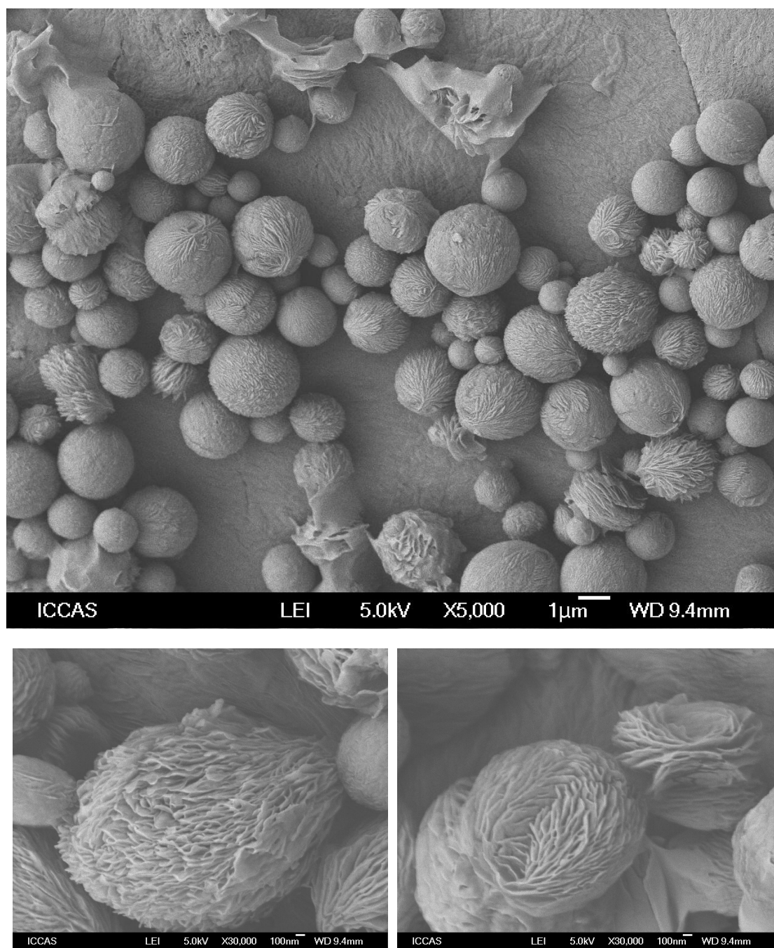
Fig. S2 SEM images of spherulites particles prepared from UHMWPE.
