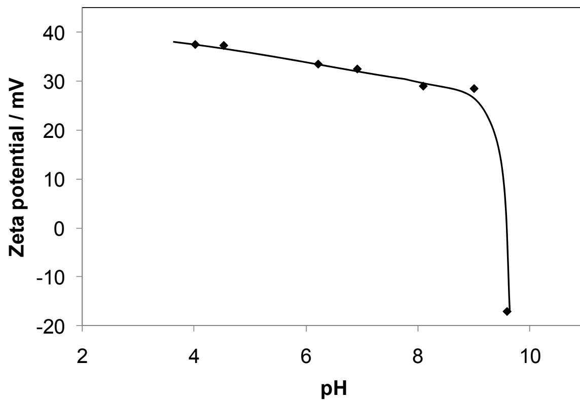
Figure caption: Evolution of zeta potential as a function of pH
