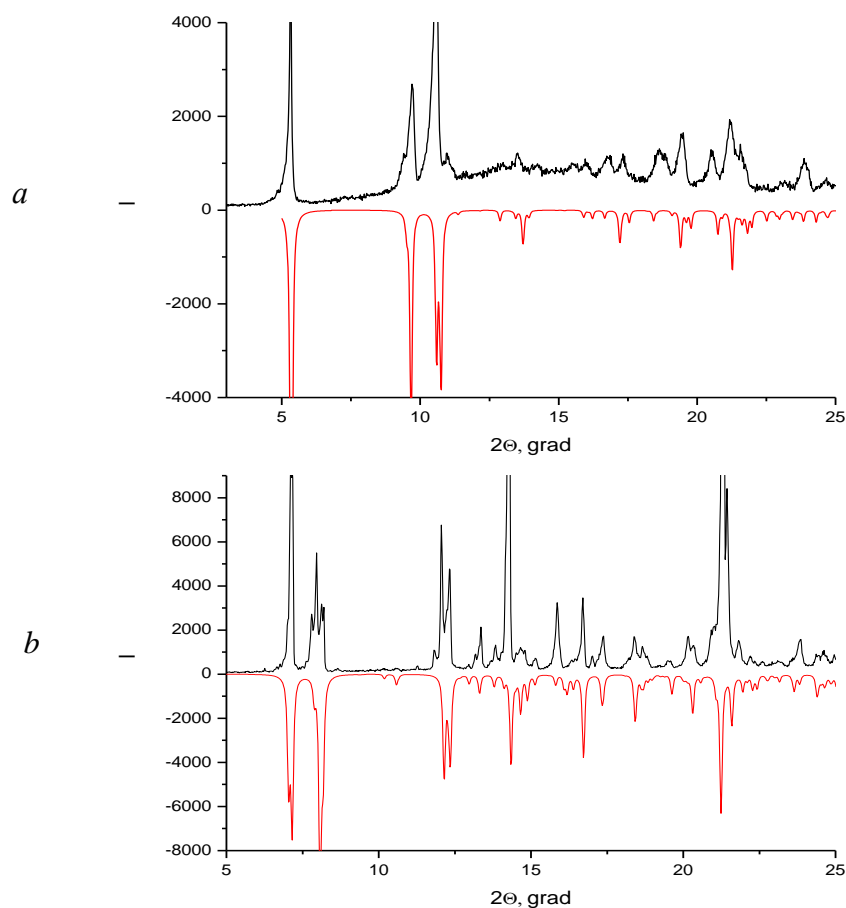
Fig. S1. A comparison of experimental XRPD plots for 1 (a), 2 (b) with those derived from single-crystal X-ray diffraction data (inverse).
