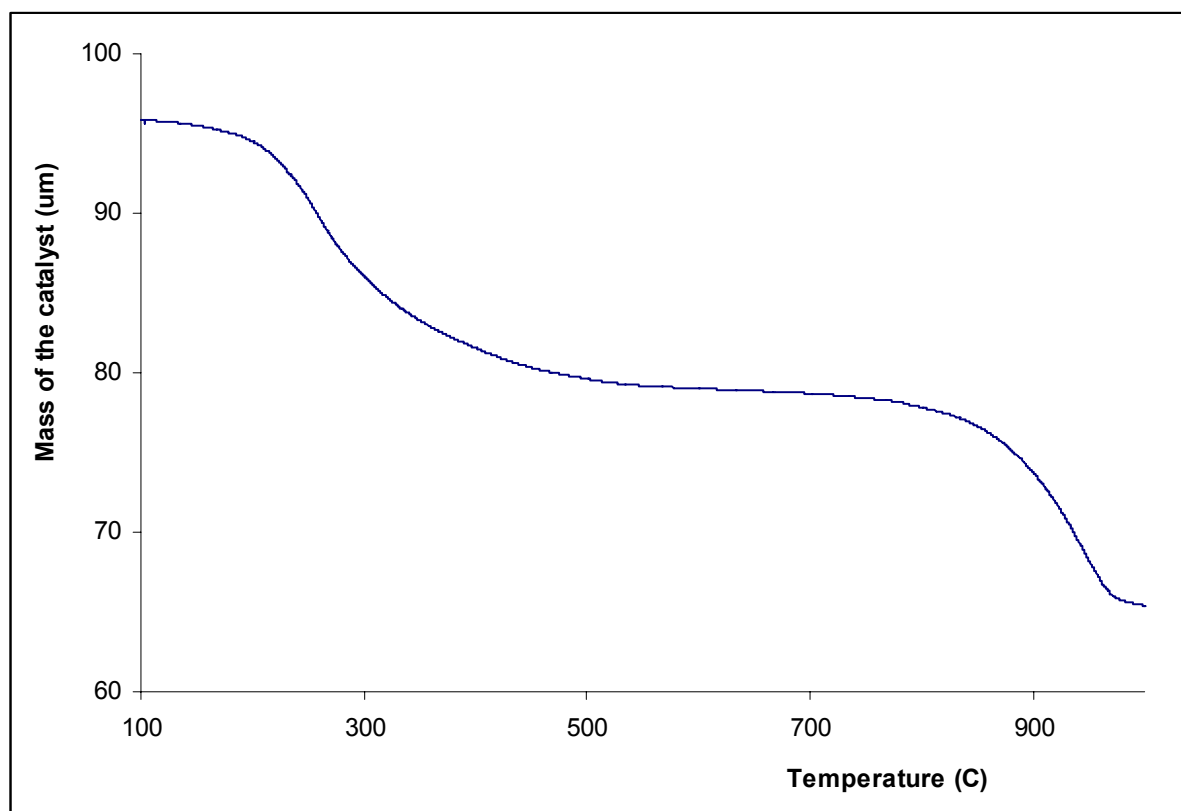
Figure S1. TGA curve of Ag/TiO 2-x N x photocatalyst
