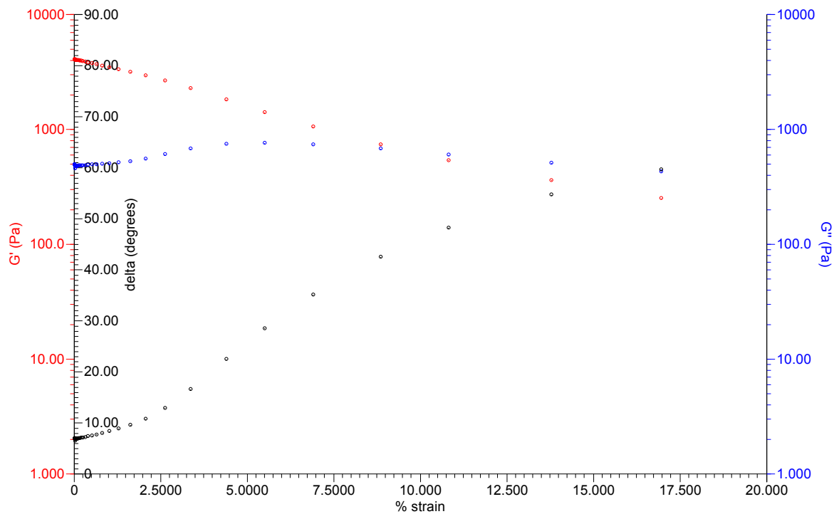
Figure S5 stress sweep rheometry for the metallogel shown in figure S4
