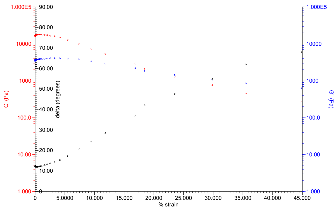
Figure S3 Strain sweep rheometry for a 1:1 mixture of \text{AgNO}_3 and \text{L}^{10} in thf / water 3:2 1 wt. %.
