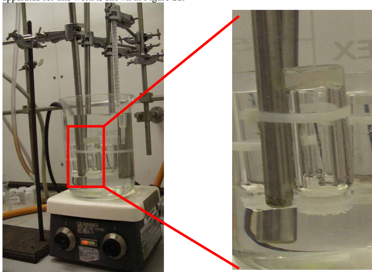
Figure S2 apparatus for T_{\text{gel}} measurements
