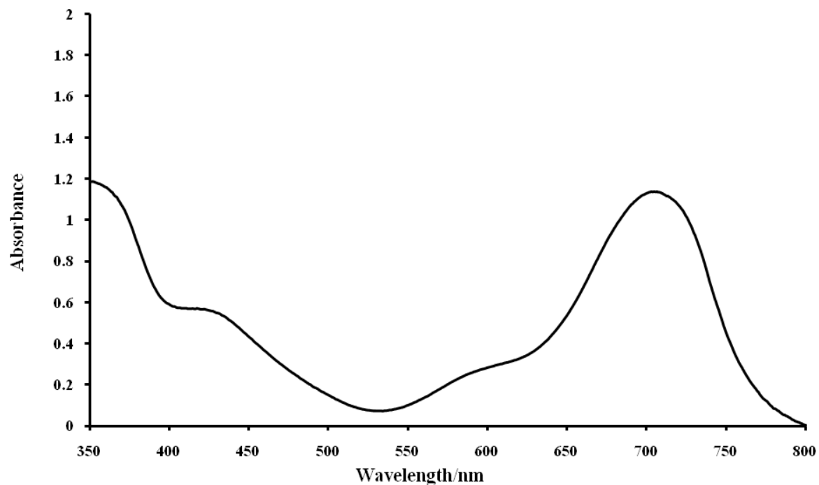
Fig. 1: UV-Vis spectrum of 5.50 \times 10^{-6} M of complex 2
