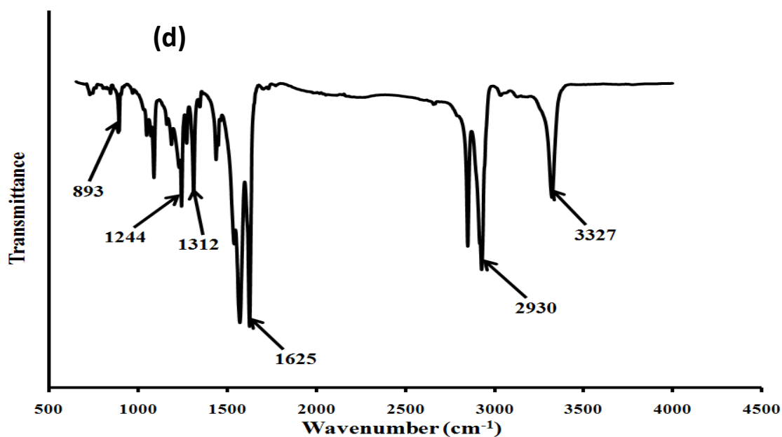
Figure 2: IR spectra of (a) SWCNT-COOH and (b) complex 2, (c) mixture of SWCNT and complex-2 and (d) SWCNT-2 nano-composite.
