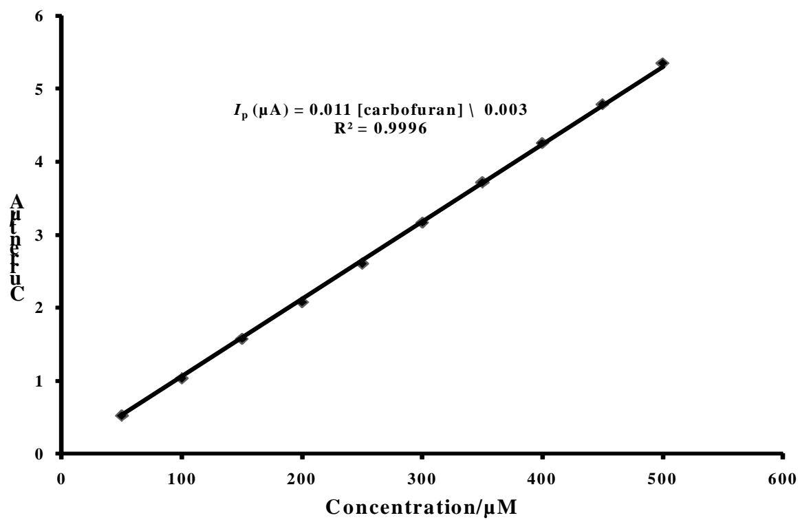
Fig. 3 Calibration curve of carbofuran on SWCNT-2-SAM
