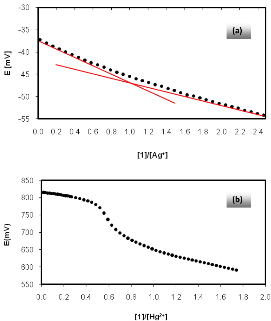
Fig. II. Potentiometric titration curves of Ag^+ (a) and Hg^{2+} (b) (as perchlorates) with 1 in acetonitrile at 298.15 K.
