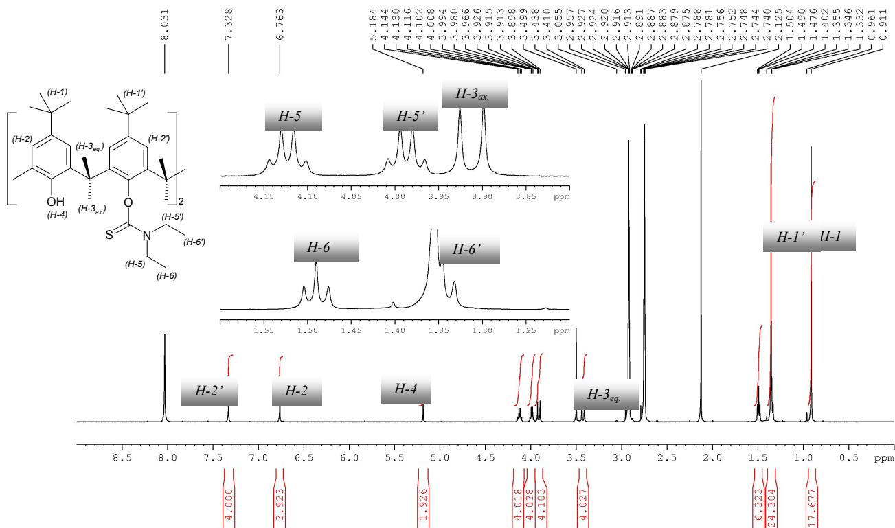
Fig. I. 1 H NMR spectra for 1 in d 7 -DMF.
