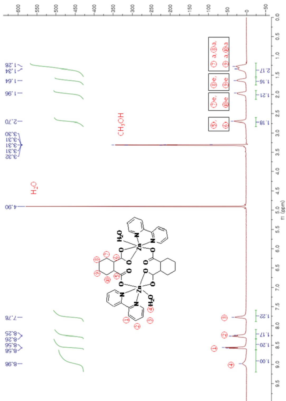
Fig. S7. 1 H NMR spectrum of 1 in CD 3 OD
