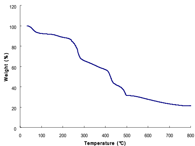
Fig S6. TGA result of 6
