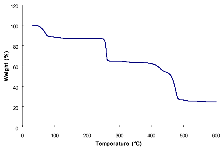
Fig S2. TGA result of 2
