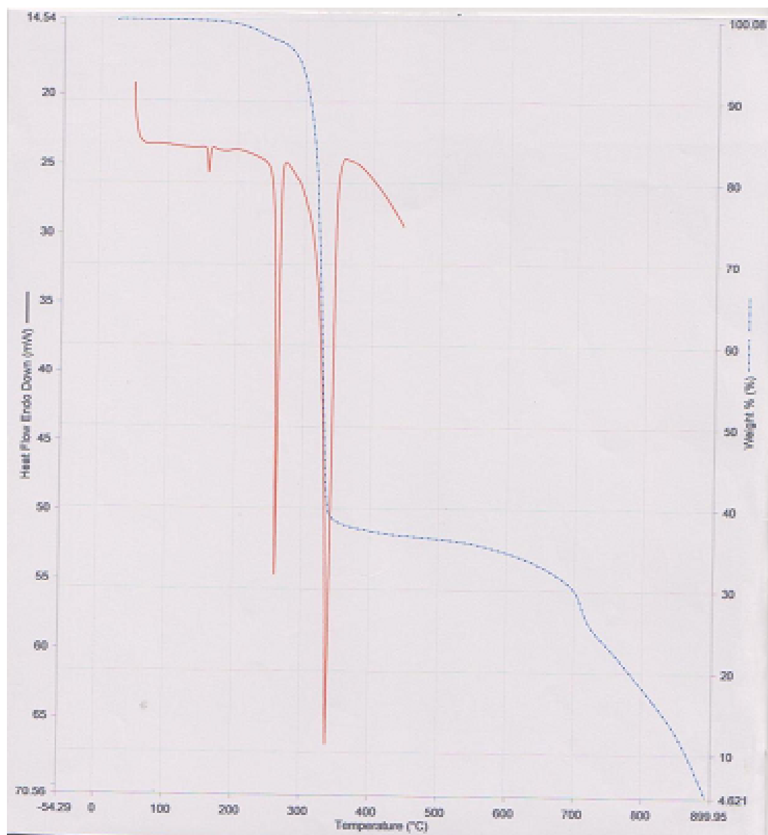
Figure 2. (a) TGA and (b) DSC thermograms of \text{Cd}(\text{pip-dtc})_2 .
