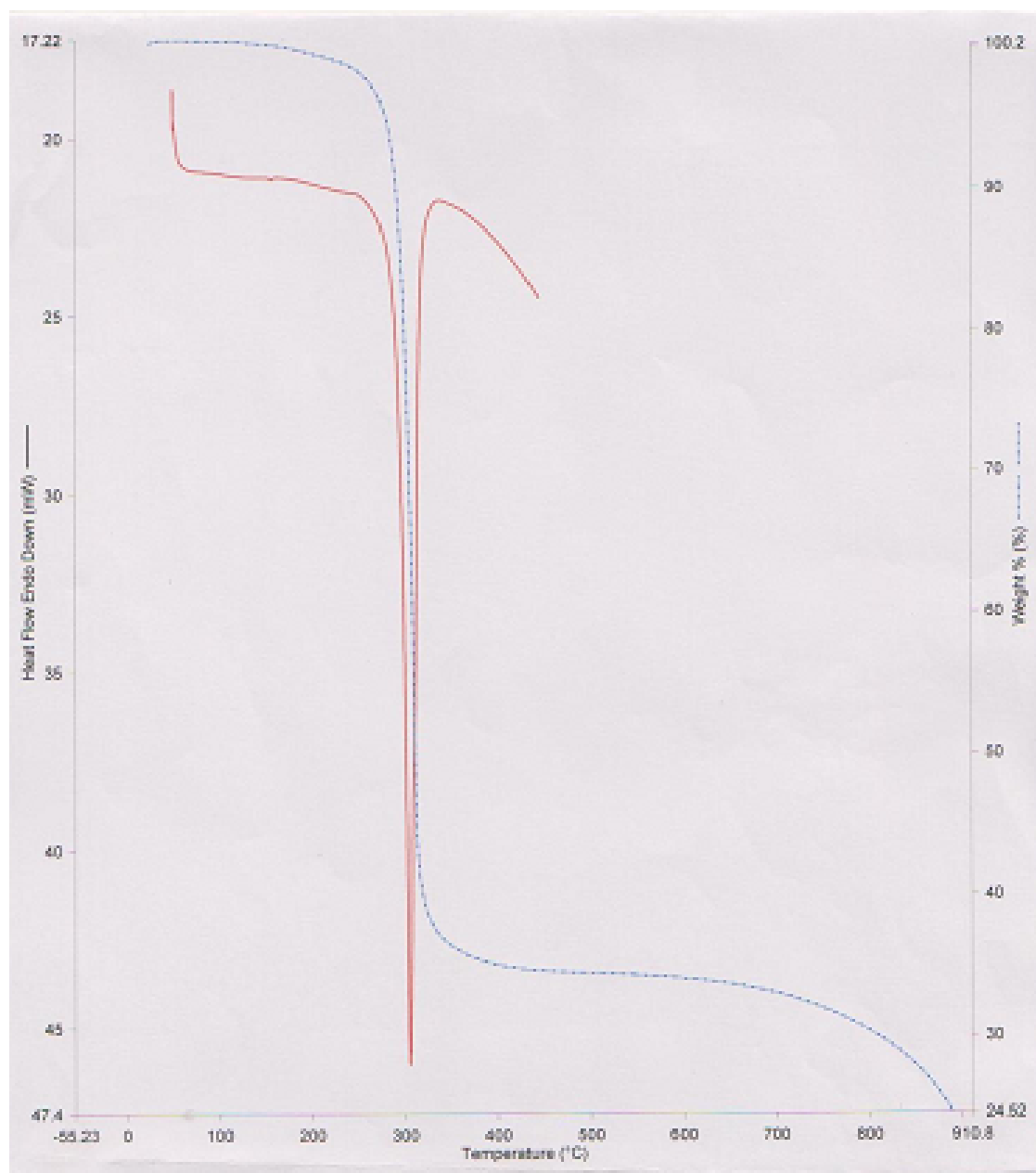
Figure 1. (a) TGA and (b) DSC thermograms of \text{Cd}(\text{thq-dtc})_2 .
