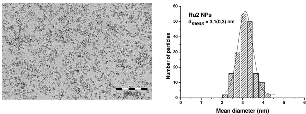
Figure S2. TEM image of N -phosphanylamidine-stabilized ruthenium nanoparticles Ru2 and the corresponding particle size distribution.
