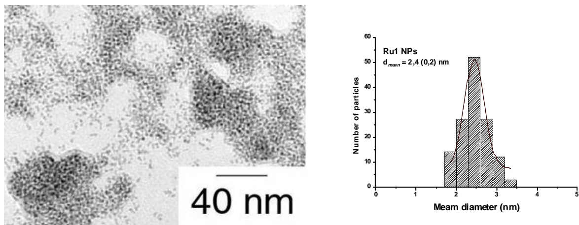
Figure S1. TEM image of N -phosphanylamidine-stabilized ruthenium nanoparticles Ru1 and the corresponding particle size distribution
