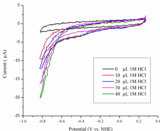
Figure S1-1. Cyclic voltammograms of a GC background 0.1 M NBu 4 BF 4 acetonitrile solution ( black ) in the presence of 10 \mu L ( red ), 20 \mu L ( blue ), 30 \mu L ( purple ) and 40 \mu L ( green ) 1 M HCl (100 mV/s). Smoothed 5 point adjusted averaging was used to remove electrical noise.
