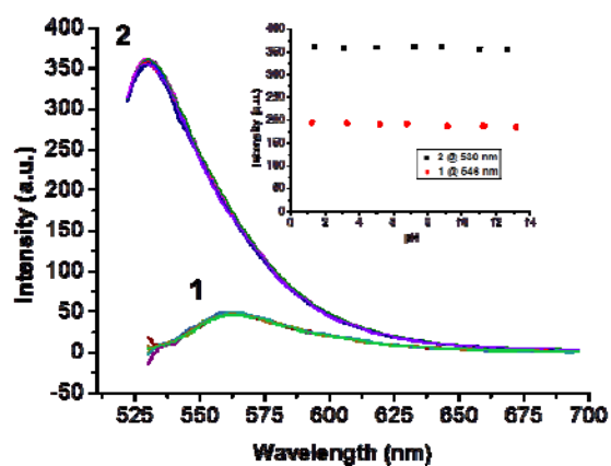
Figure 1S: Emission spectra of 1 and 2 (50 μM) vs pH (pH adjusted by HCl or NaOH) in THF-water (85:15 v/v) solution ( \lambda_{\text{ex}} = 502 \text{ nm} ).
